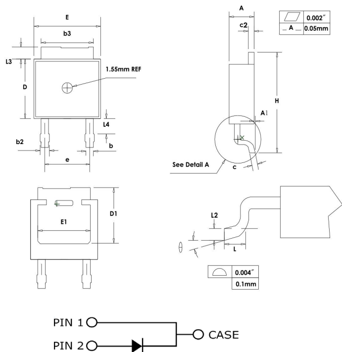
Package TO-252-2
