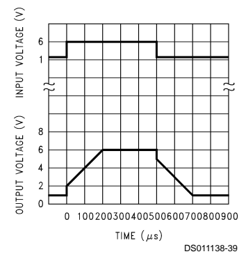
Non-Inverting Large Signal Pulse Response ( A_V = +1 )
