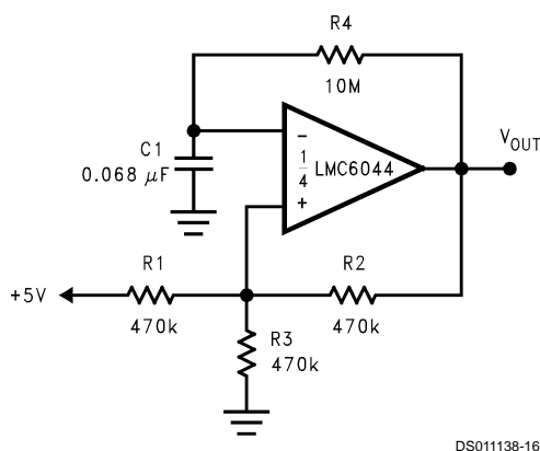
FIGURE 11. 1 Hz Square-Wave Oscillator
