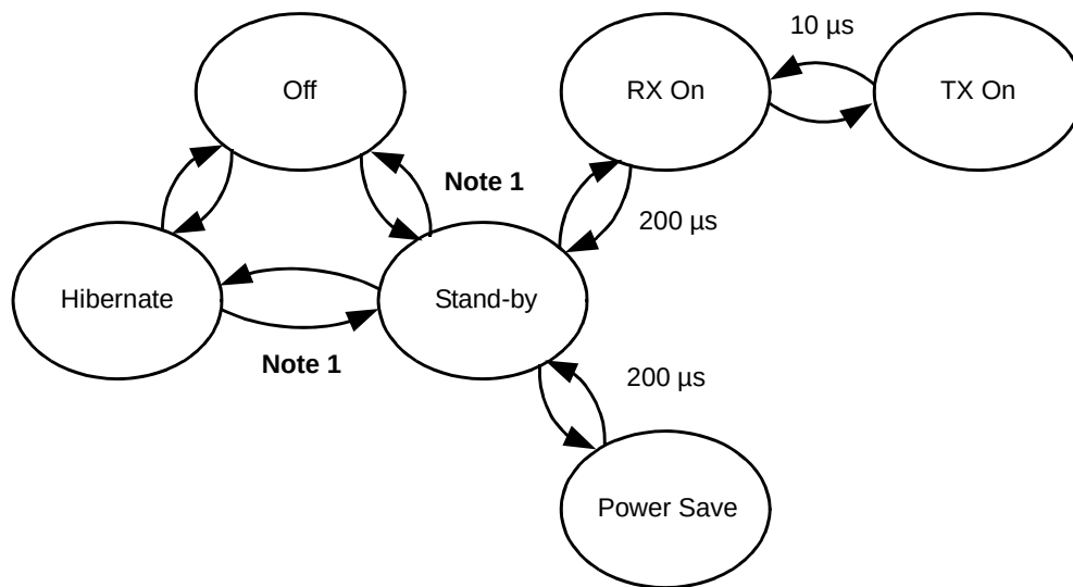
FIGURE 2-3: MRF24WG0MA/MB POWER-STATE DIAGRAM
