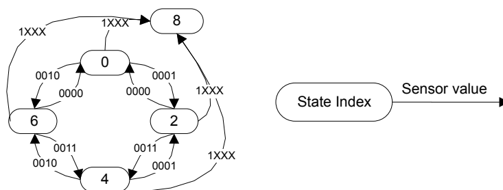
Figure 29.19. FSM Example 2
