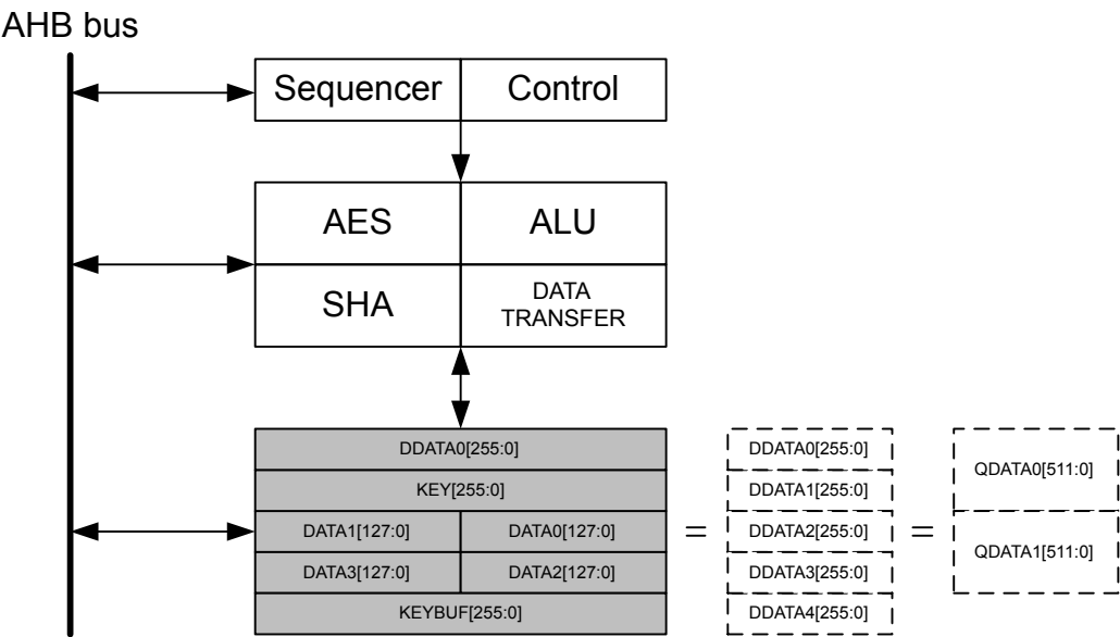
Figure 32.1. CRYPTO Overview
