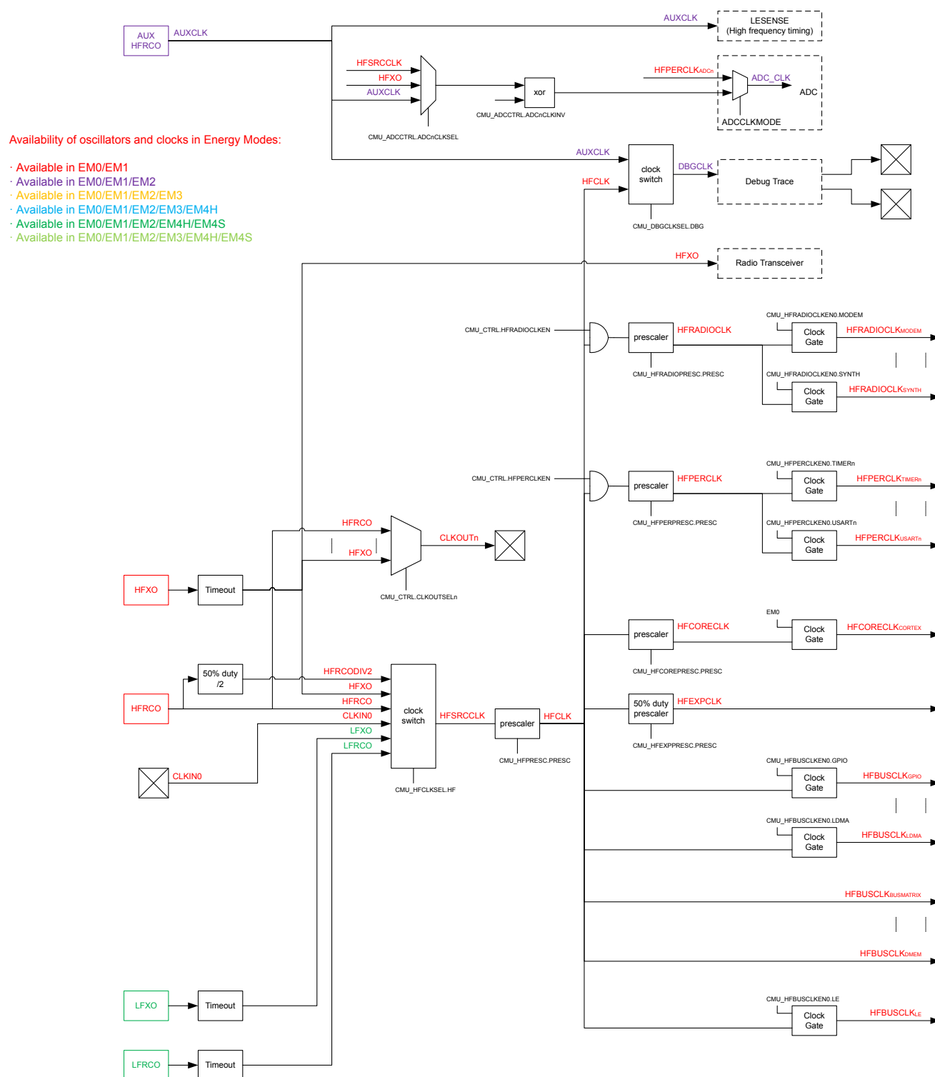
Figure 12.1. CMU Overview - High Frequency Portion
