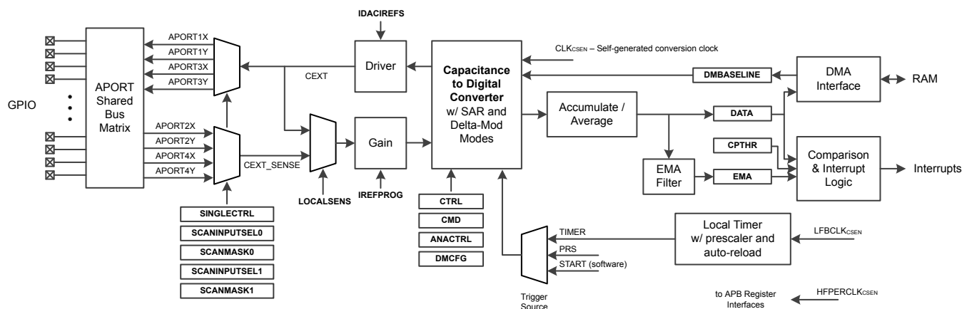
Figure 35.1. CSEN Overview
