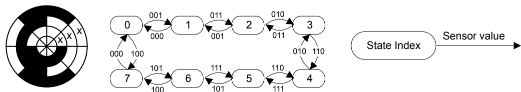
Figure 29.18. FSM Example 1
