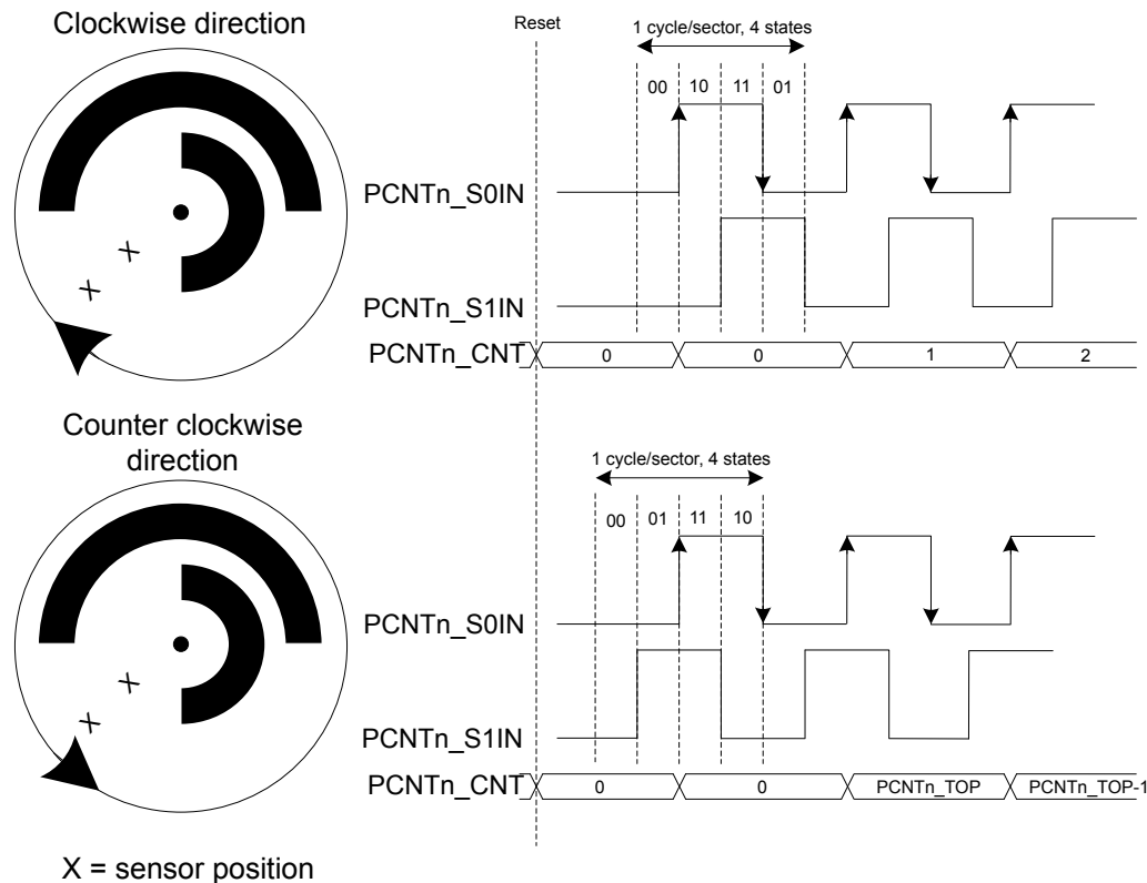
Figure 17.2. PCNT Quadrature Coding
