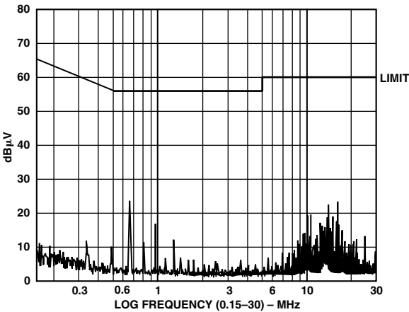
Figure 15. Conducted Emissions
