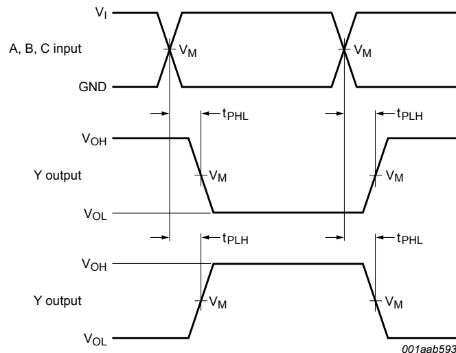
Figure 15. Input A, B and C to output Y propagation delay times
