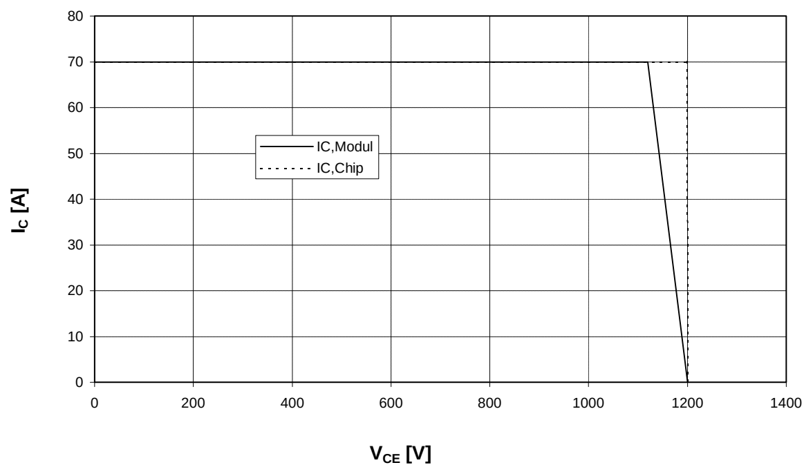
Reverse bias safe operating area Inverter (RBSOA) T_{vj} = 125^\circ\text{C} , V_{GE} = \pm 15\text{V} , R_G = 22\ \Omega
