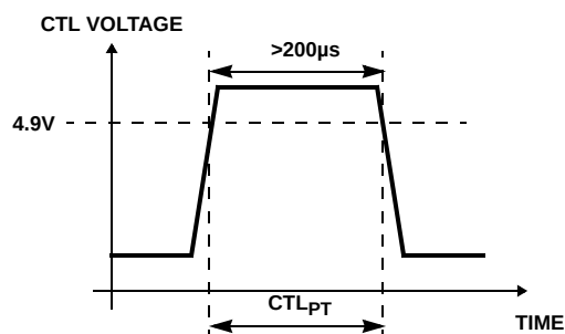
FIGURE 2. EEPROM PROGRAMMING
