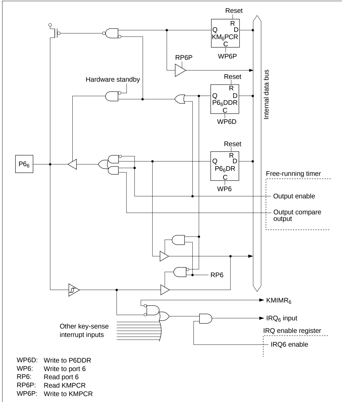
Figure C.6 (c) Port 6 Block Diagram (Pin P6 6 )
