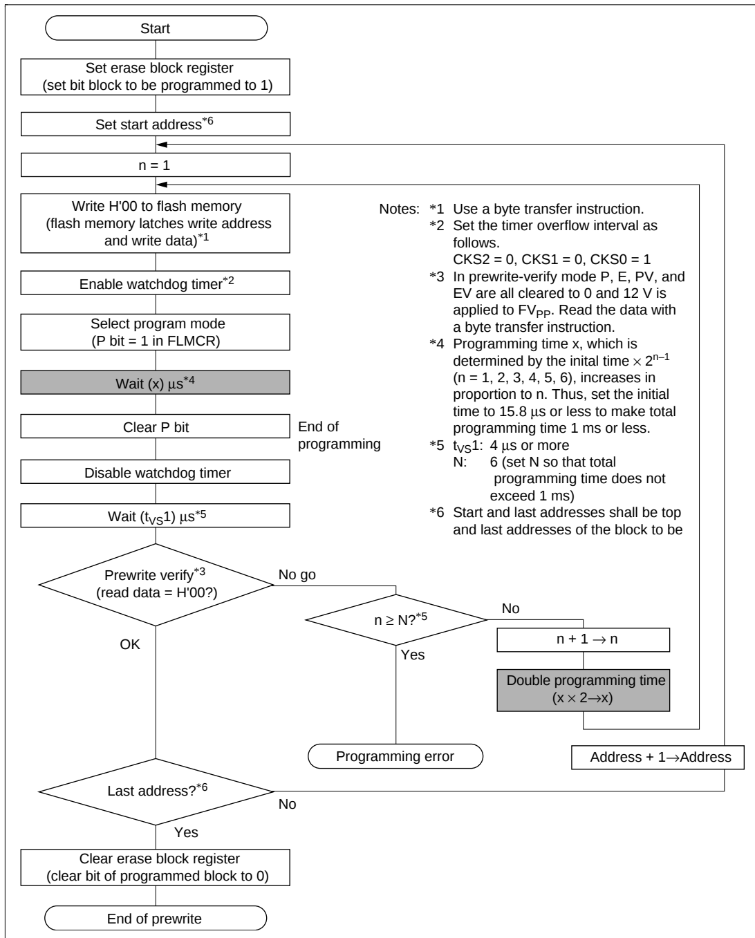
Figure 20.10 Prewrite Flowchart
