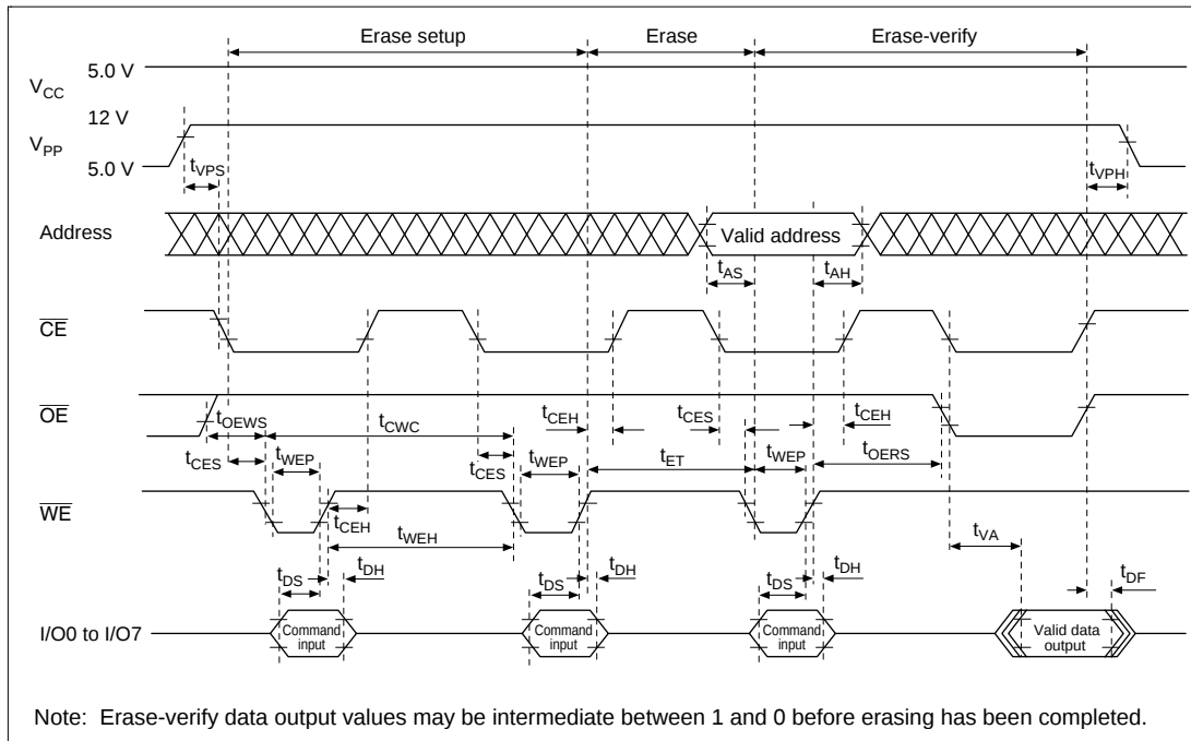
Figure 19.19 Erase Timing
