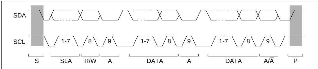
Figure 13.5 I²C Bus Timing
