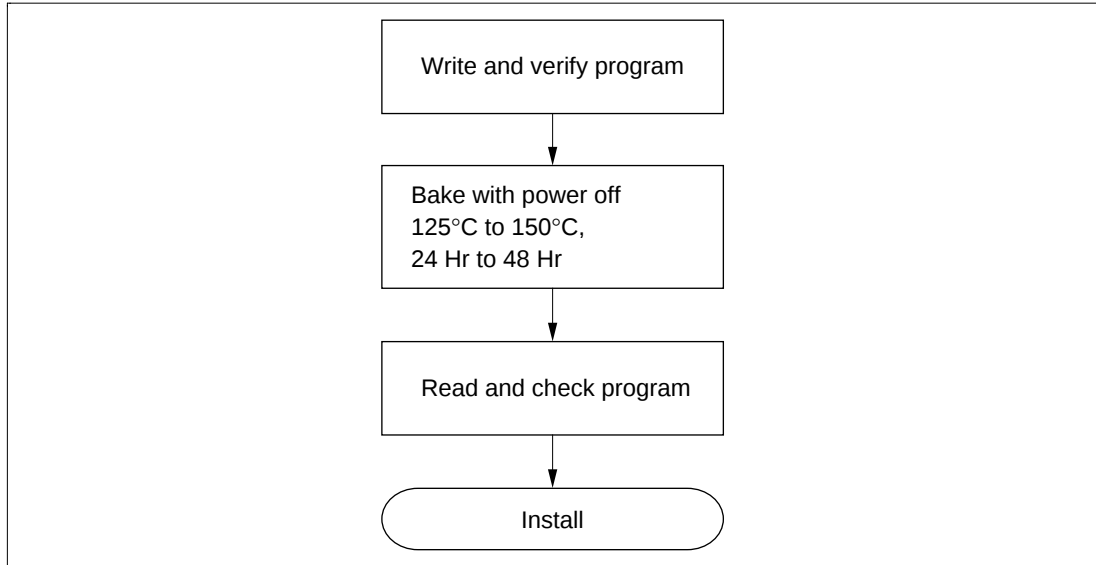
Figure 18.7 Recommended Screening Procedure
