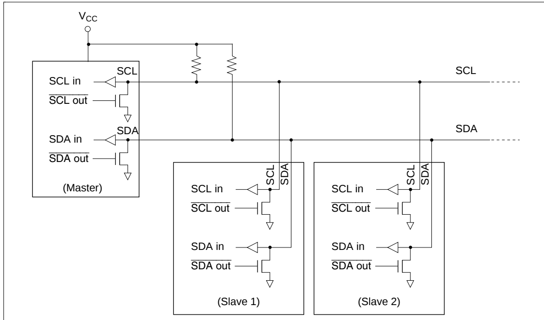
Figure 13.1 I²C Bus Interface Connections (Example) (H8/3337 Series Chip as Master)
