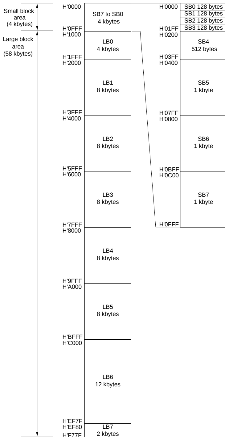
Figure 20.2 Erase Block Map
