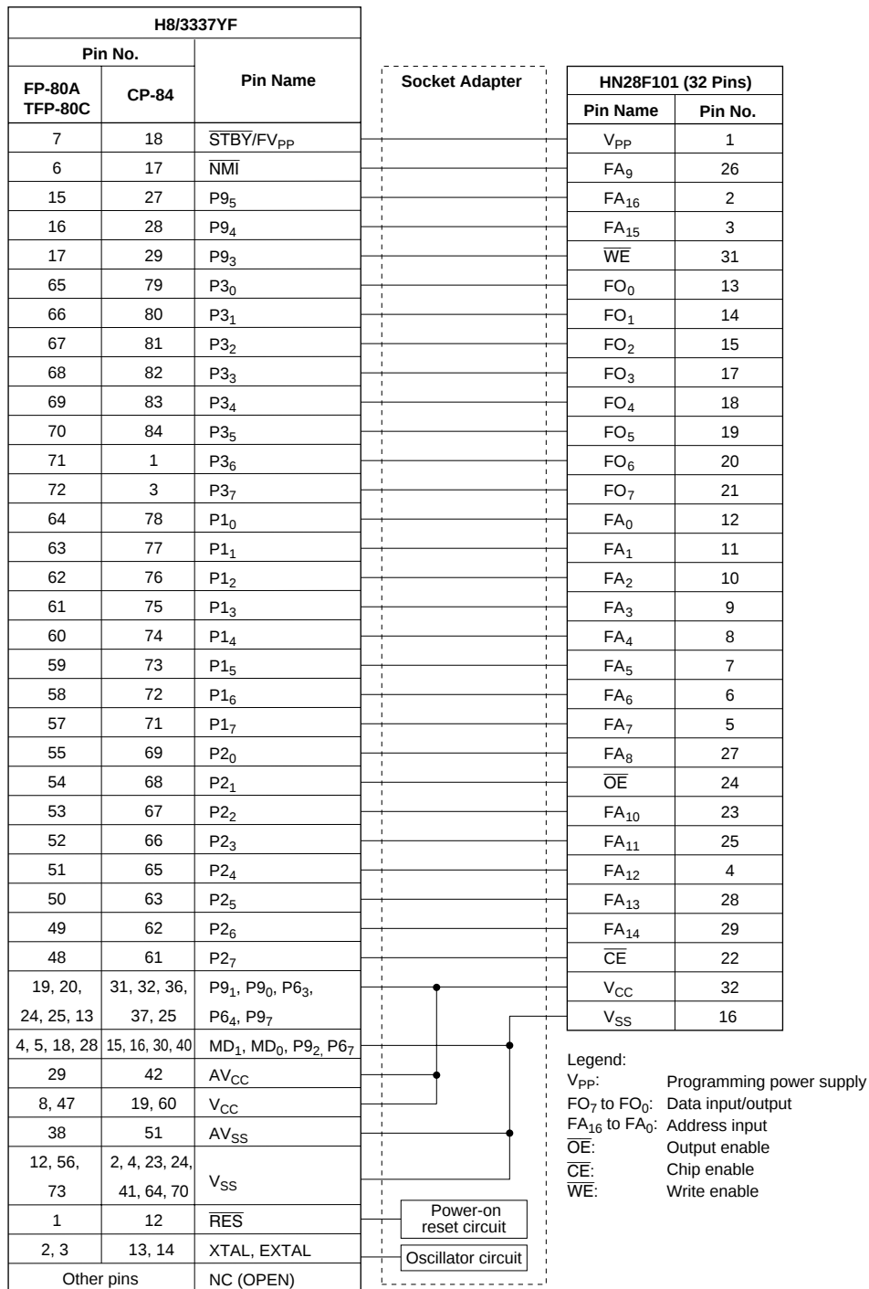
Figure 20.14 Wiring of Socket Adapter
