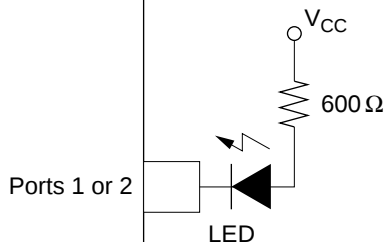
Figure 23.5 Example of Circuit for Driving an LED (5-V Version)
