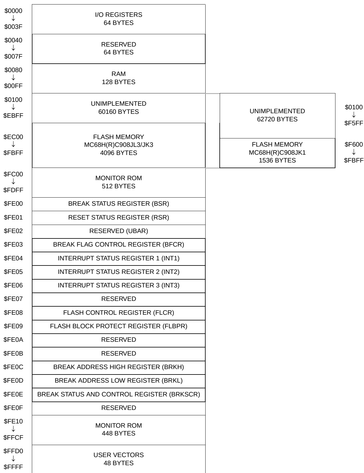
Figure 2-1. Memory Map
