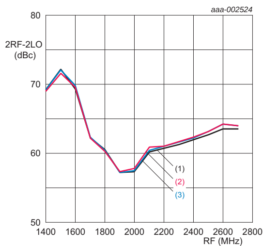
Fig 17. 2RF-2LO response versus f_{RF} and P_{i(lo)}
