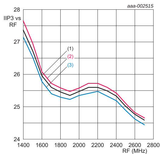
Fig 8. IIP3_i versus f_{RF} and P_{i(lo)}
