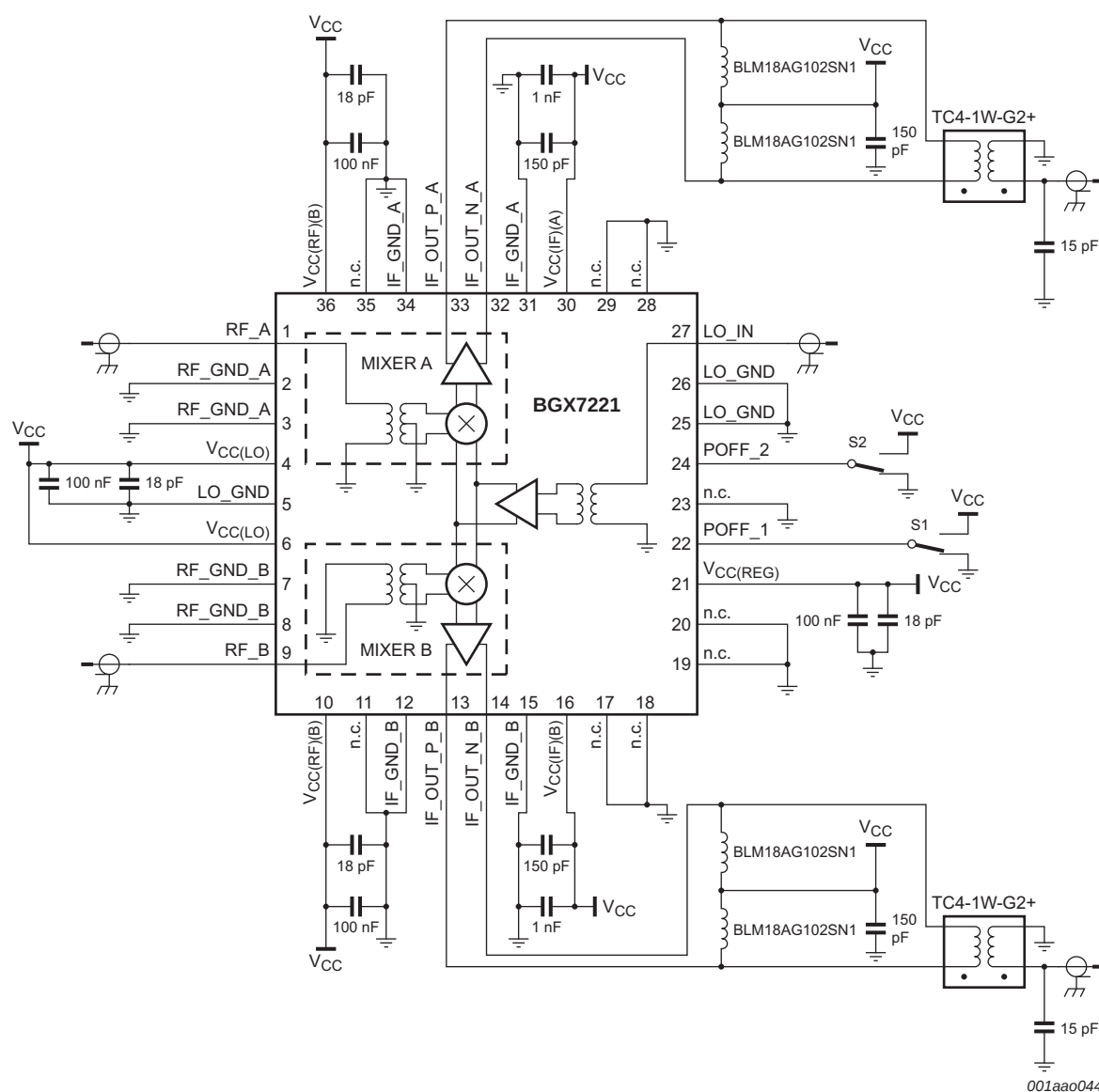
Fig 3. Application diagram
