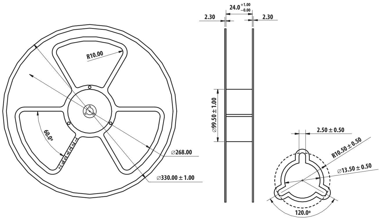
Figure 20. Reel dimensions.
