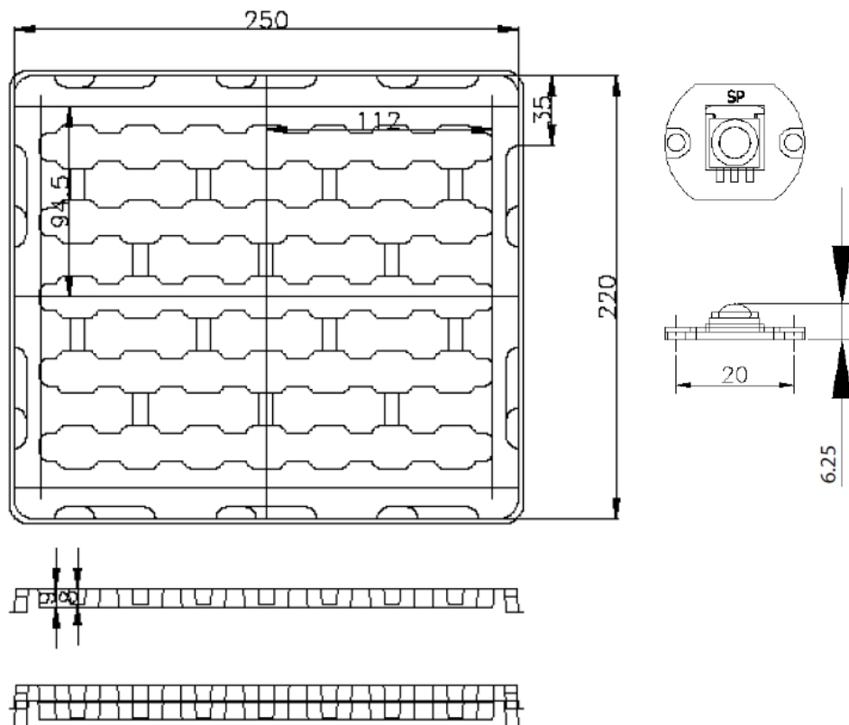
Figure 21. Tray dimensions.
