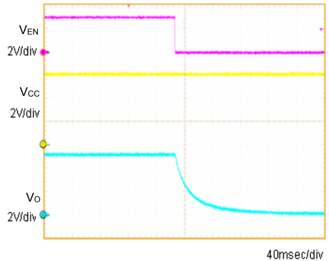
Fig.8 OFF sequence 2 Co=1μF
