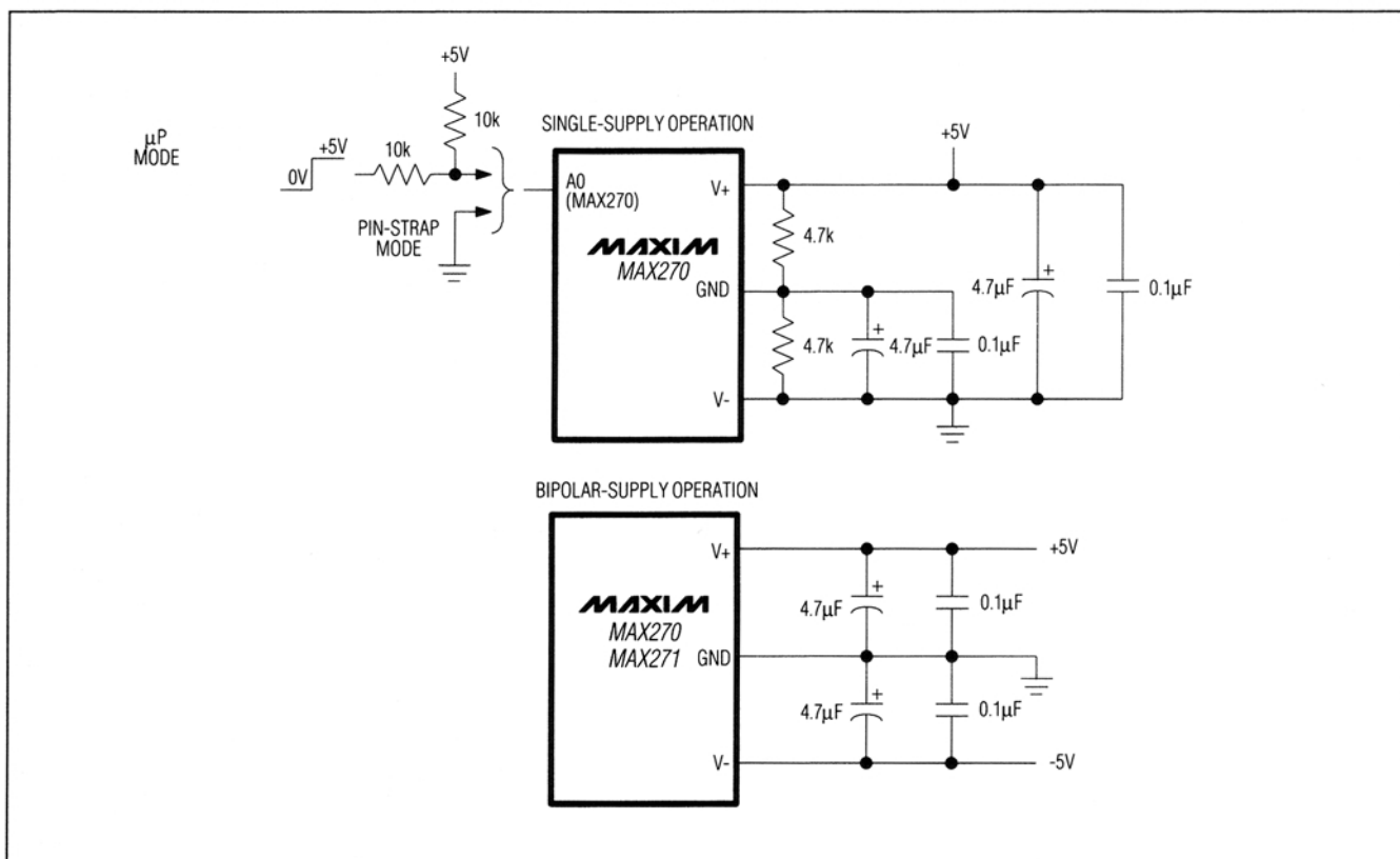
Figure 4. Power-Supply Configurations
