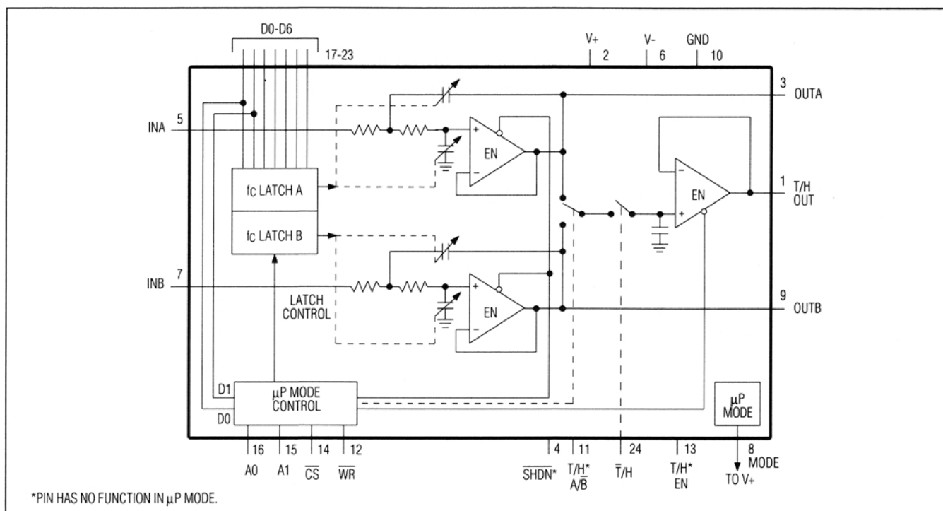
Figure 1b. MAX271 Block Diagram - \mu P Mode
