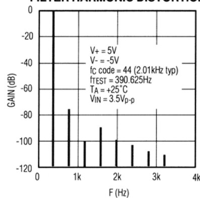
FILTER HARMONIC DISTORTION
