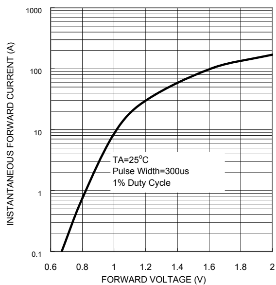
FIG. 5- TYPICAL INSTANTANEOUS FORWARD CHARACTERISTICS
