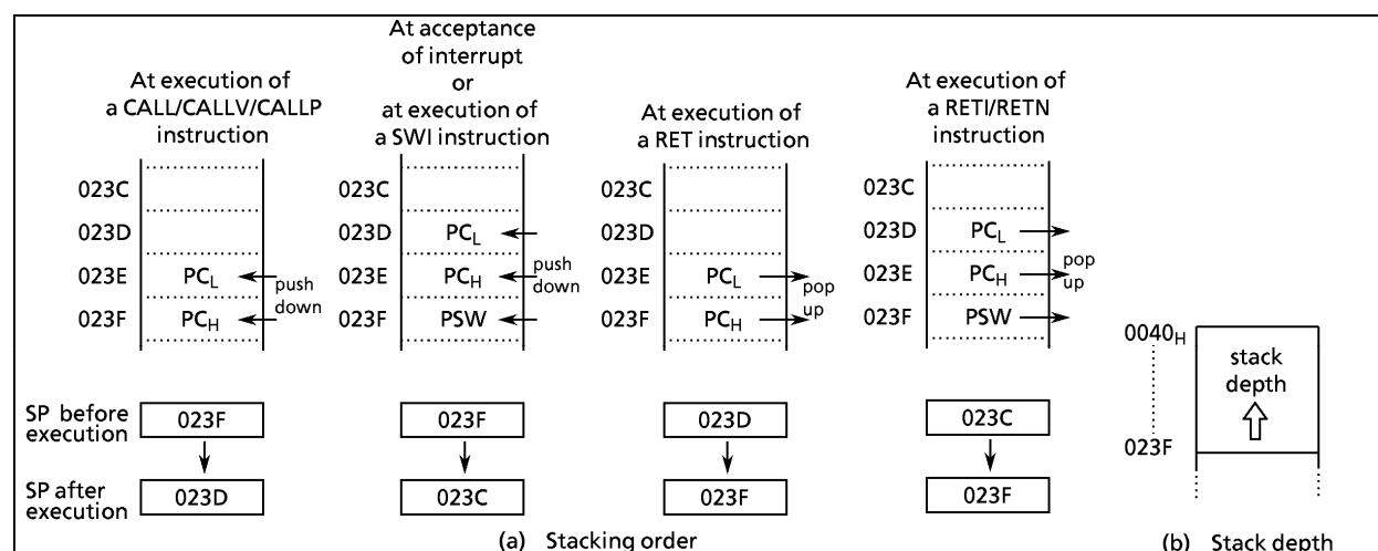
Figure 1-9. Stack
