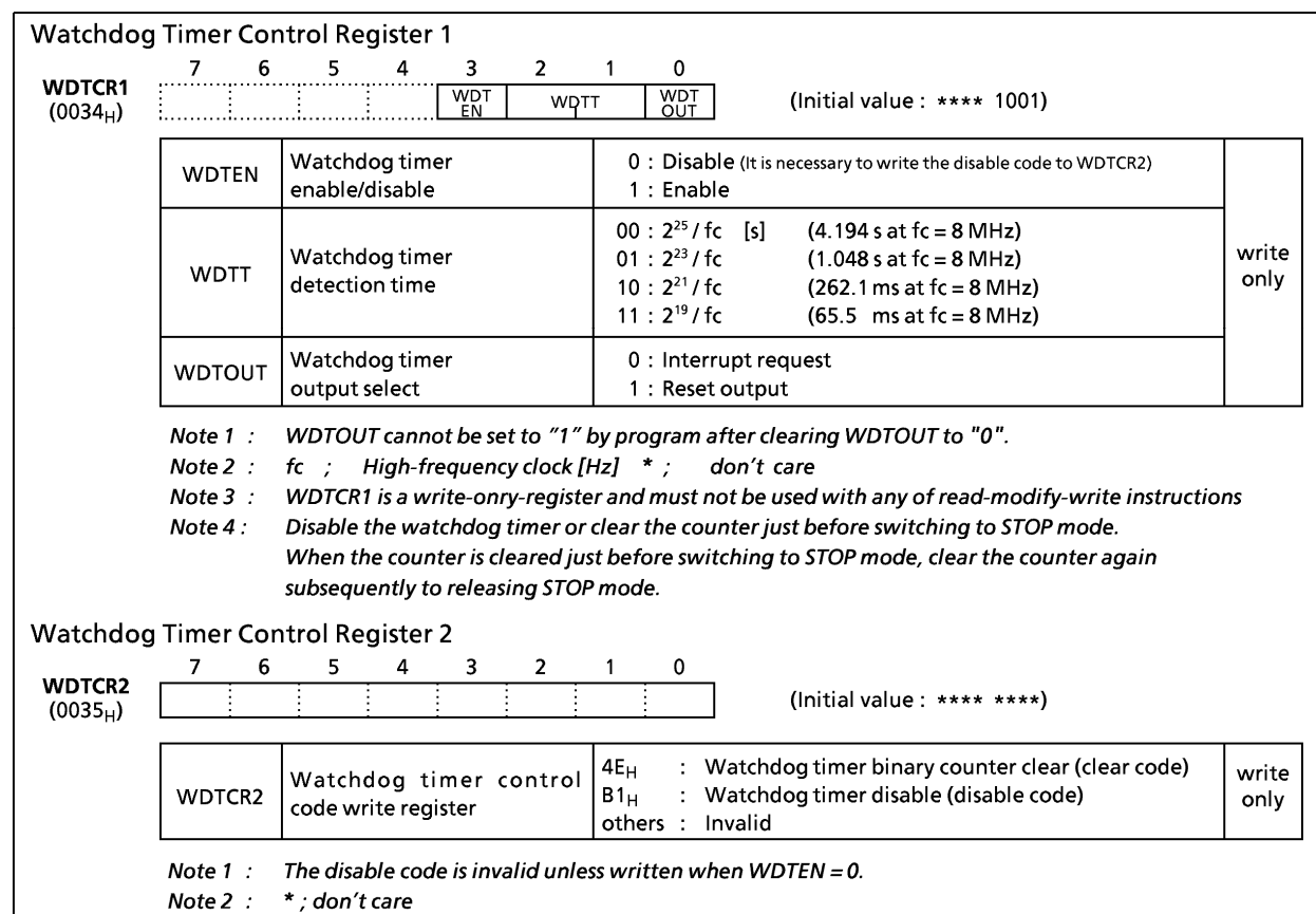
Figure 1-27. Watchdog timer control registers
