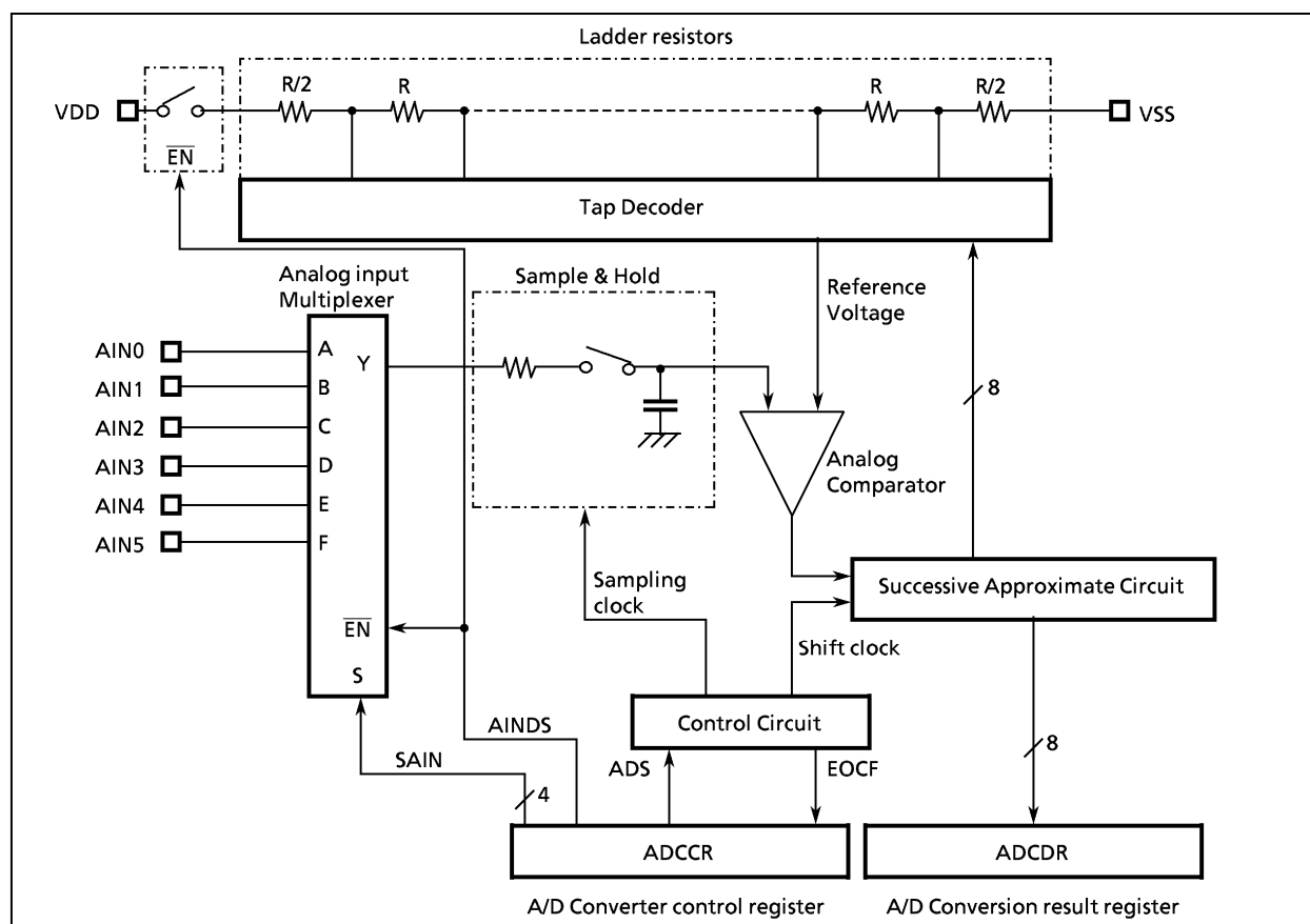
Figure 2-60. A/D converter
