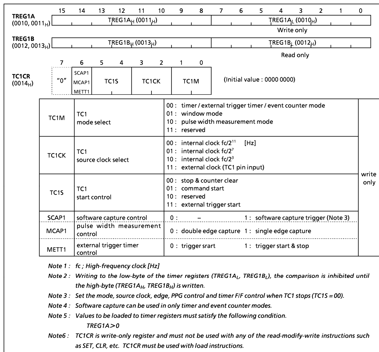
figure 2-13. Timer registers and TC1 control register
