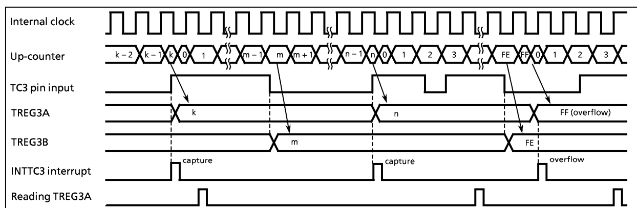
Figure 2-24. Timing chart for capture mode (TC3ES = 0)
