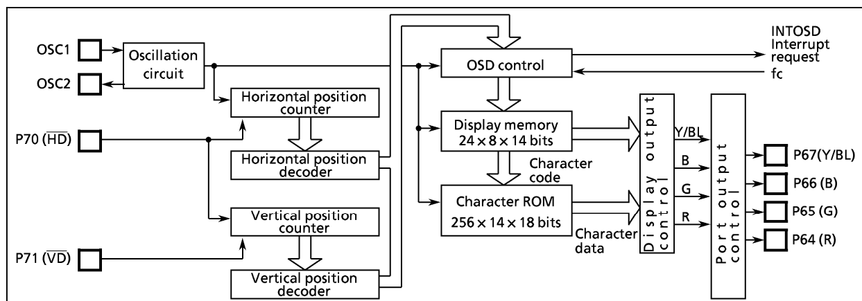
Figure 2-70. OSD circuit
