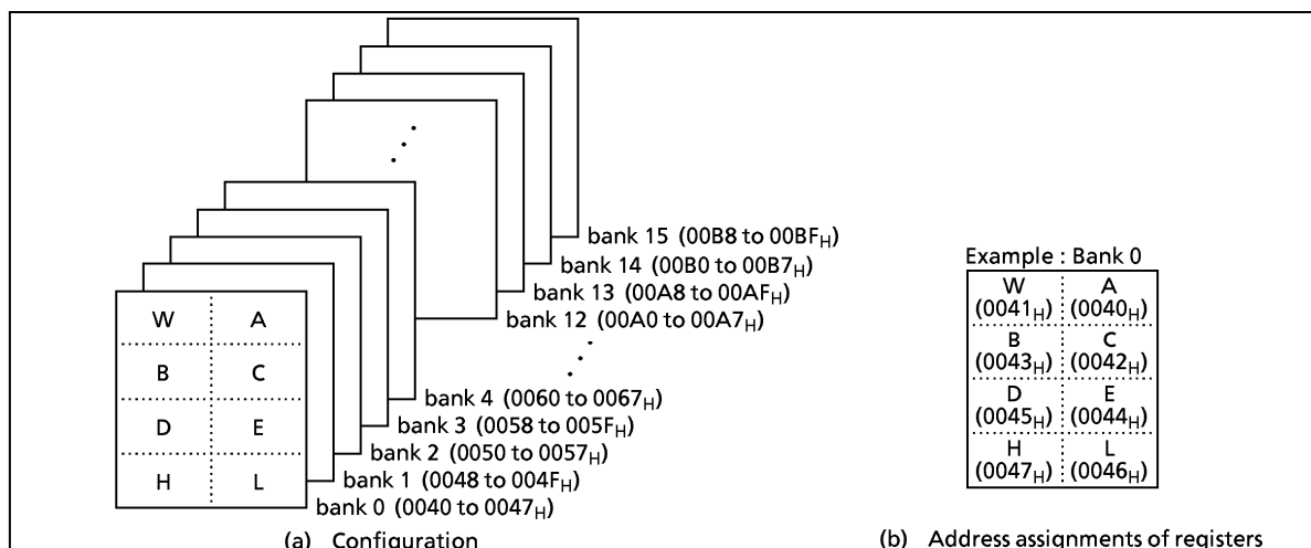
Figure 1-6. General-purpose register banks
