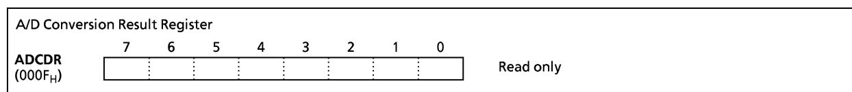
Figure 2-61. A/D conversion result register
