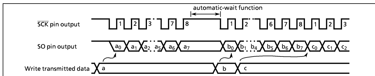
Figure 2-44. Automatic-wait function
