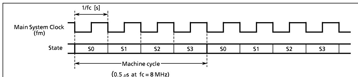
Figure 1-13. Machine cycle
