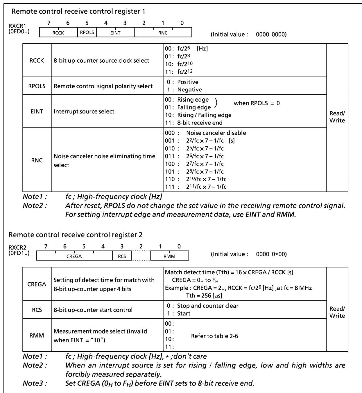
Figure 2-53. Remote control receive control register 1, 2
