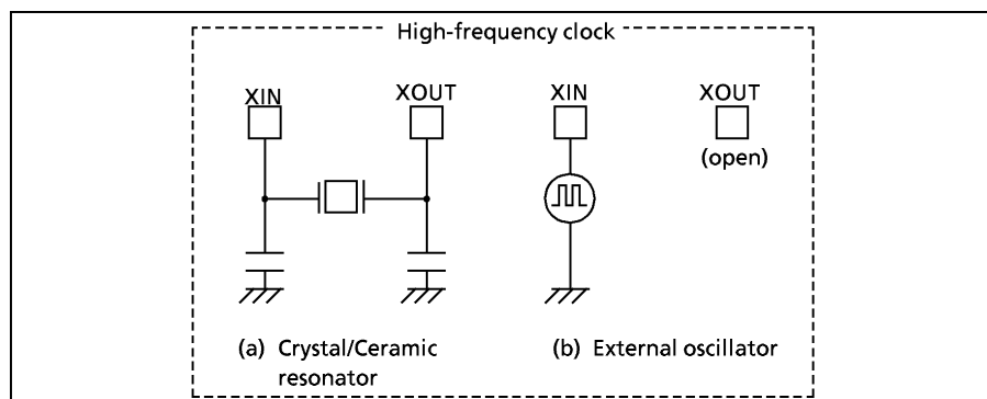
Figure 1-11. Examples of Resonator Connection
