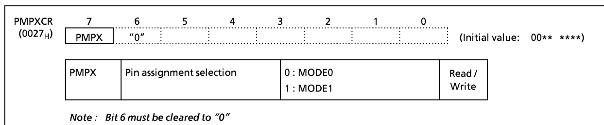
Figure 2-9. Port switching register
