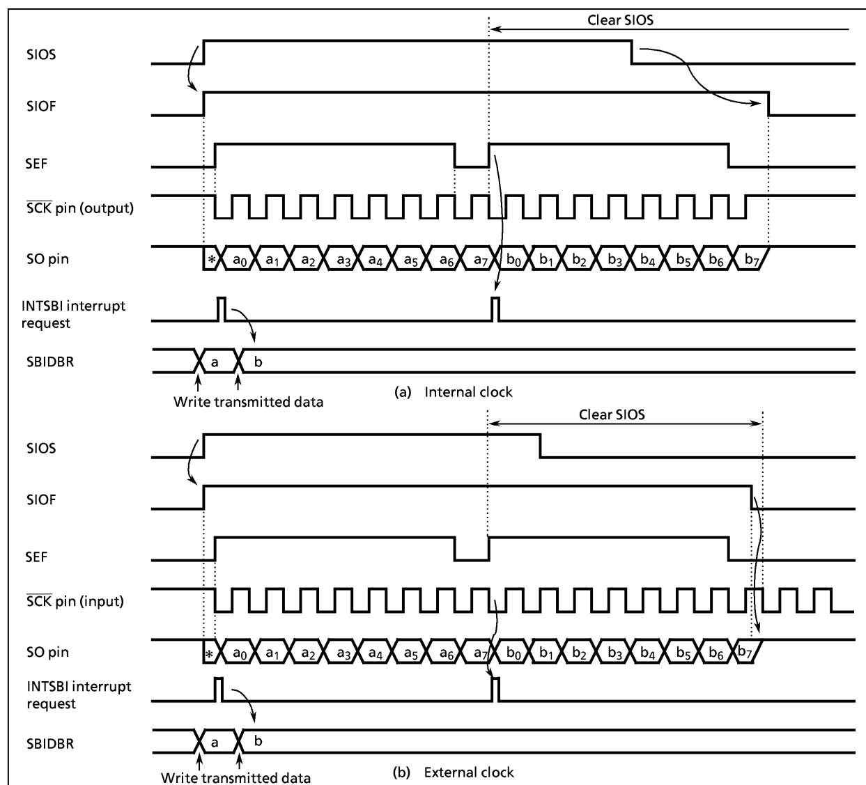
Figure 2-47. Transfer mode
