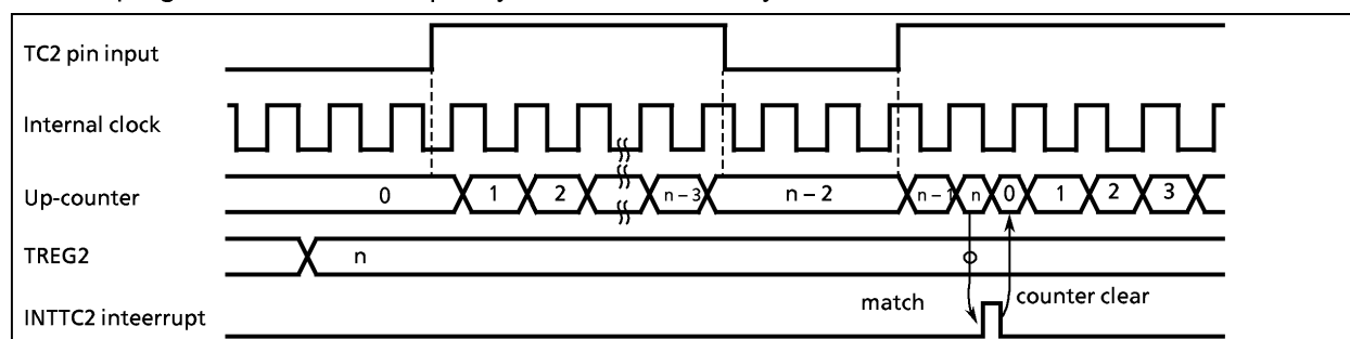
Figure 2-21. Window mode timing chart
