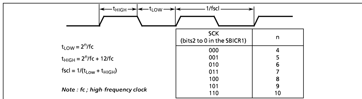
Figure 2-31. Clock source
