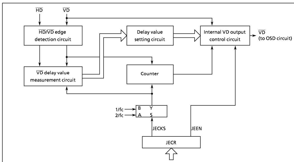
Figure 2-77. Jitter elimination circuit
