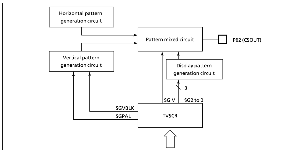
Figure 2-68. Test video signal output circuit
