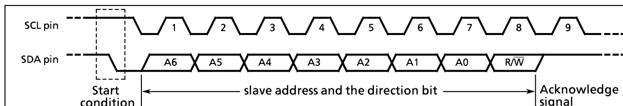
Figure 2-33. Start condition generation and slave address generation
