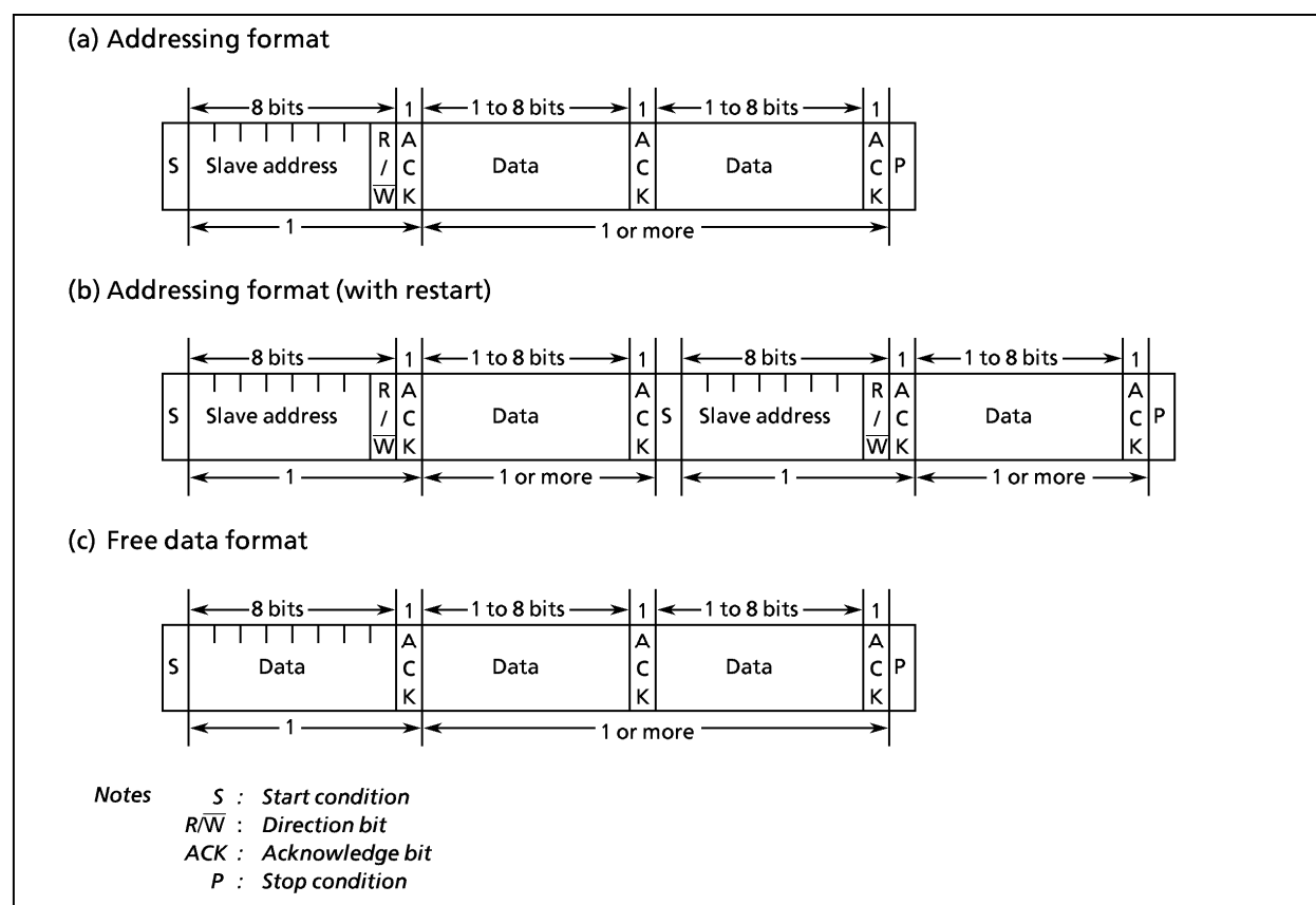
Figure 2-28. Data format
