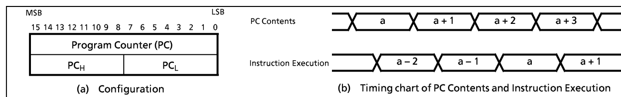
Figure 1-4. Program counter
