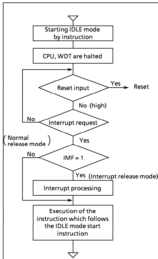
Figure 1-19. IDLE mode
