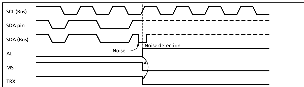
Figure 2-35. Noise detection monitor
