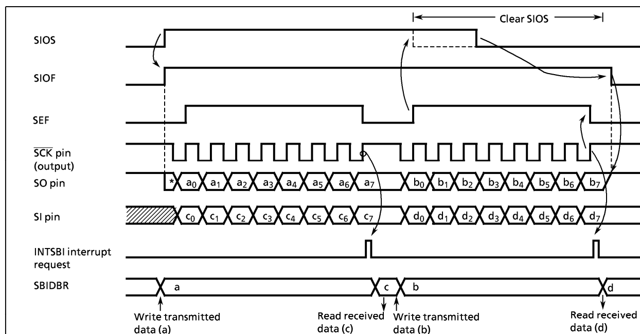
Figure 2-50. Transmit / receive mode (Example : Internal clock)
