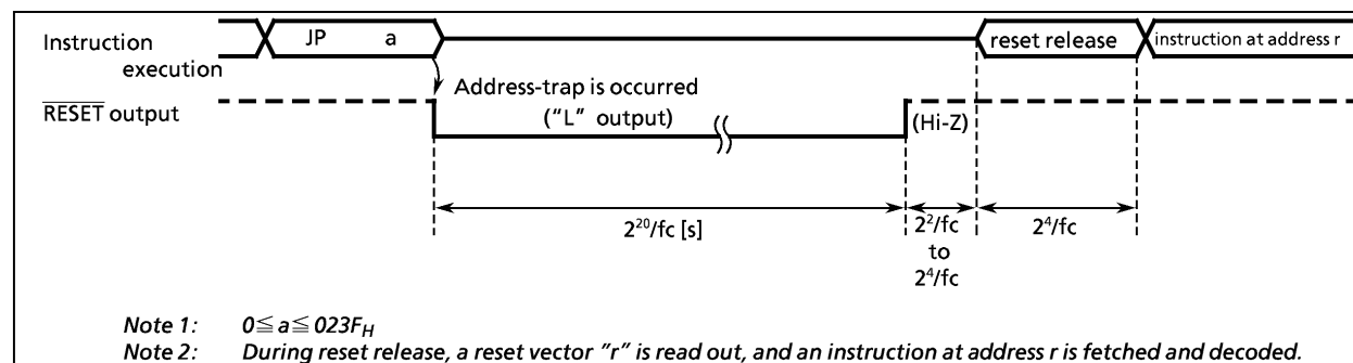
Figure 1-30. Address-trap-reset
