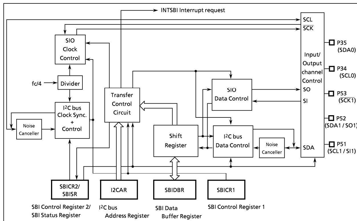
Figure 2-27. Serial bus interface (SBI-ver.A)
