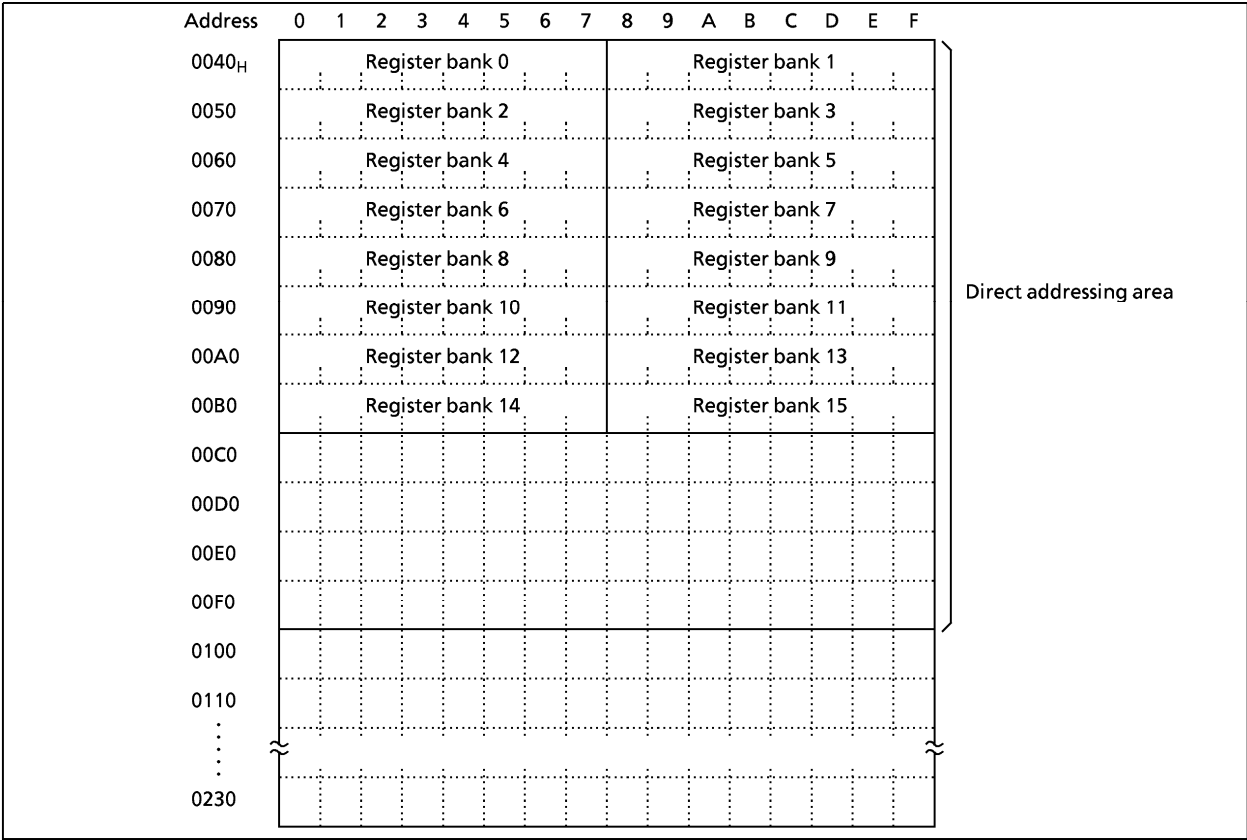
Figure 1-5. Data memory map
