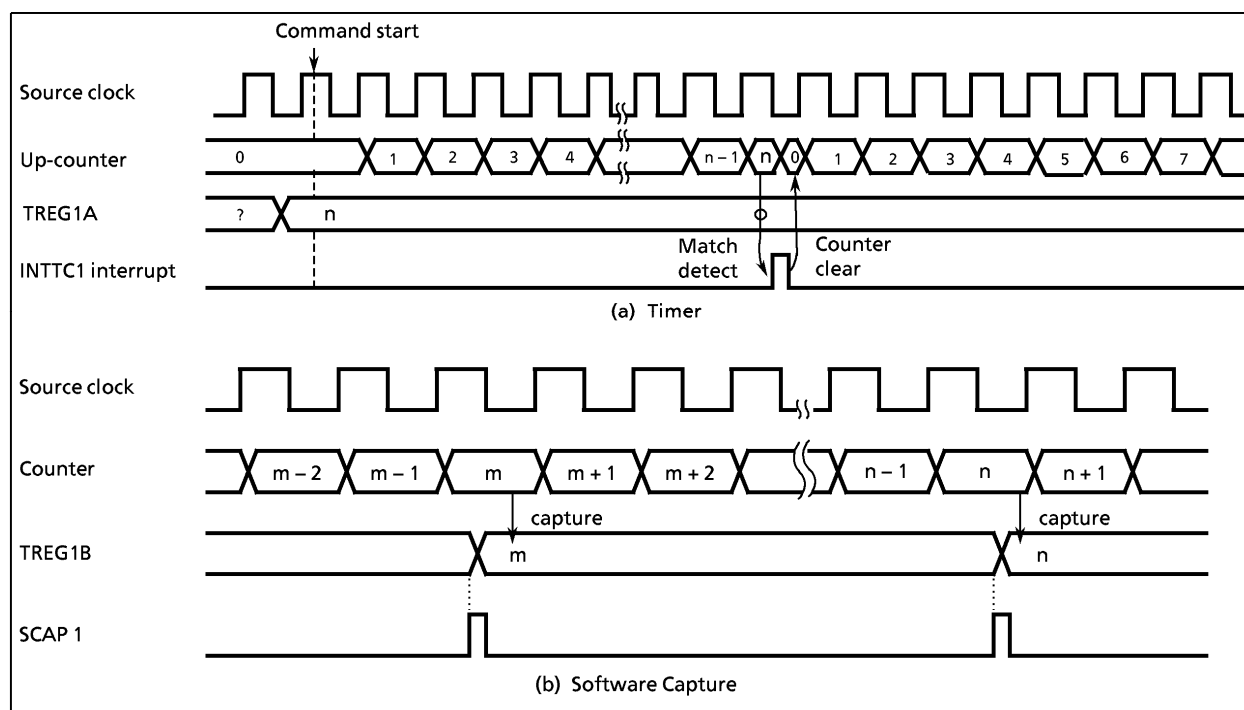
Figure 2-14. Timer mode timing chart
