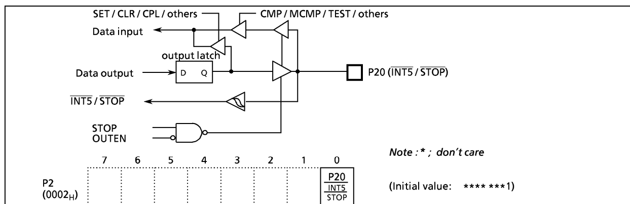
Figure 2-3. Port P2
