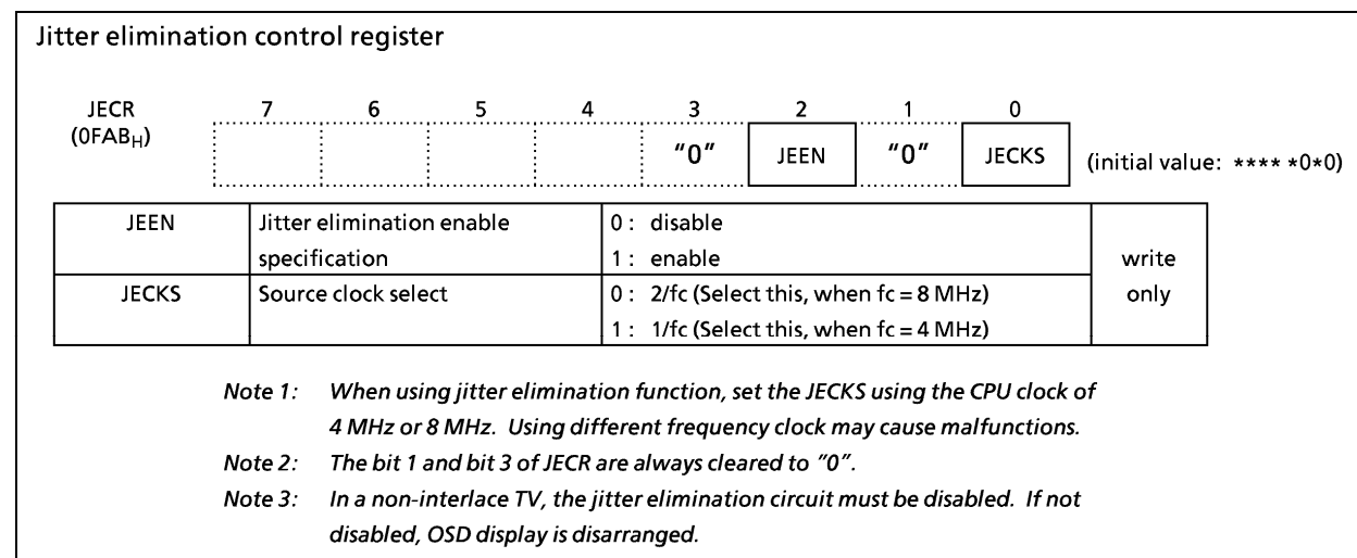
Figure 2-77. Jitter elimination control register
