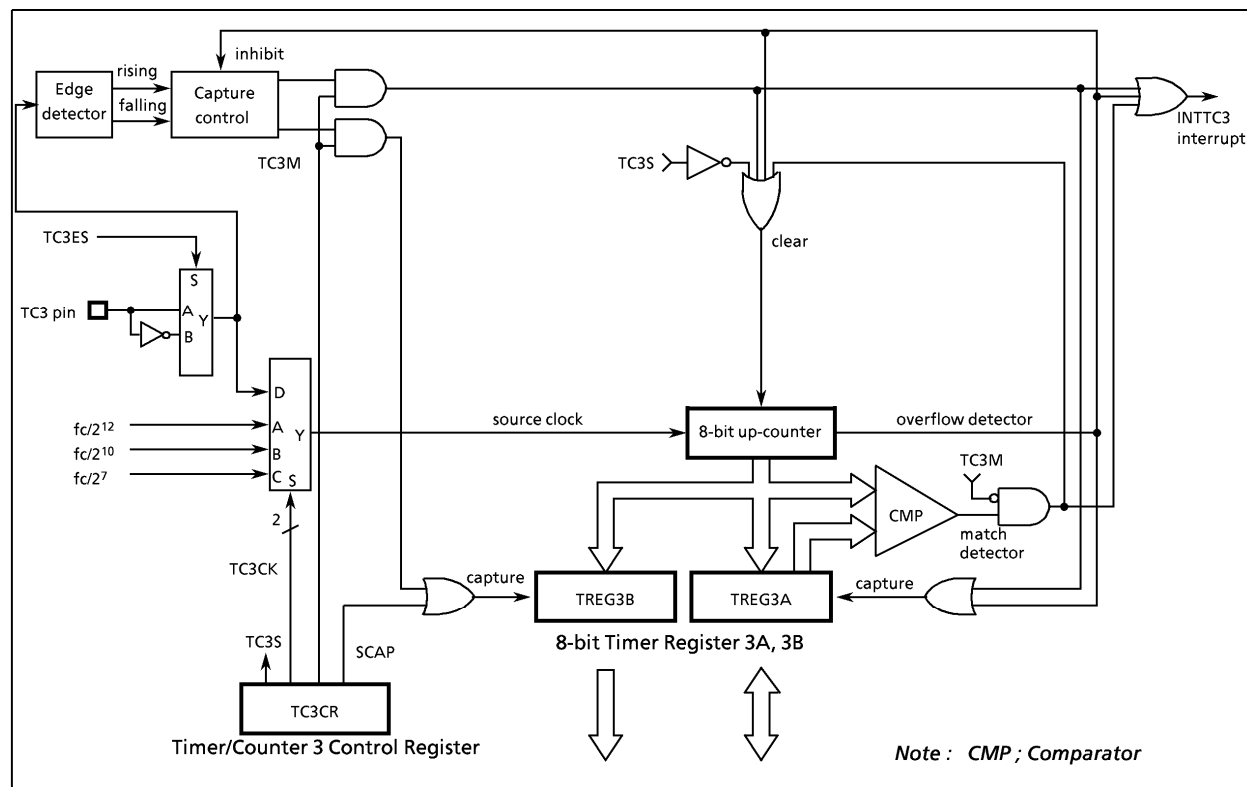
Figure 2-22. Timer/counter (TC3)
