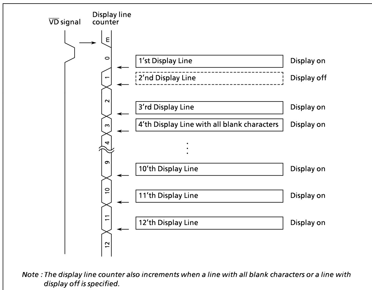
Figure 2-76. Display line counter
