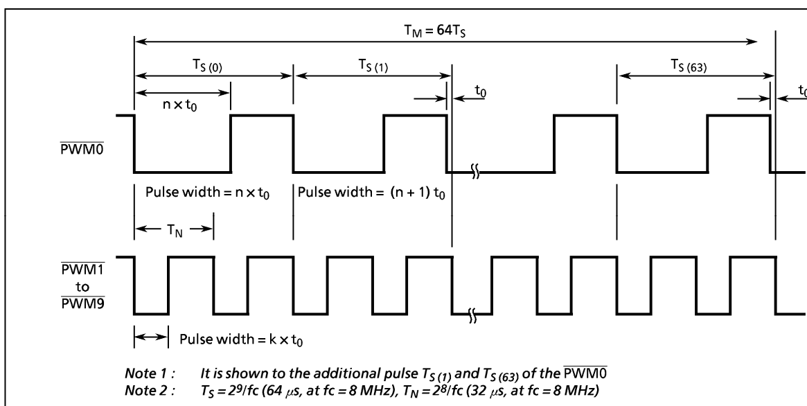
Figure 2-66. PWM output wave form
