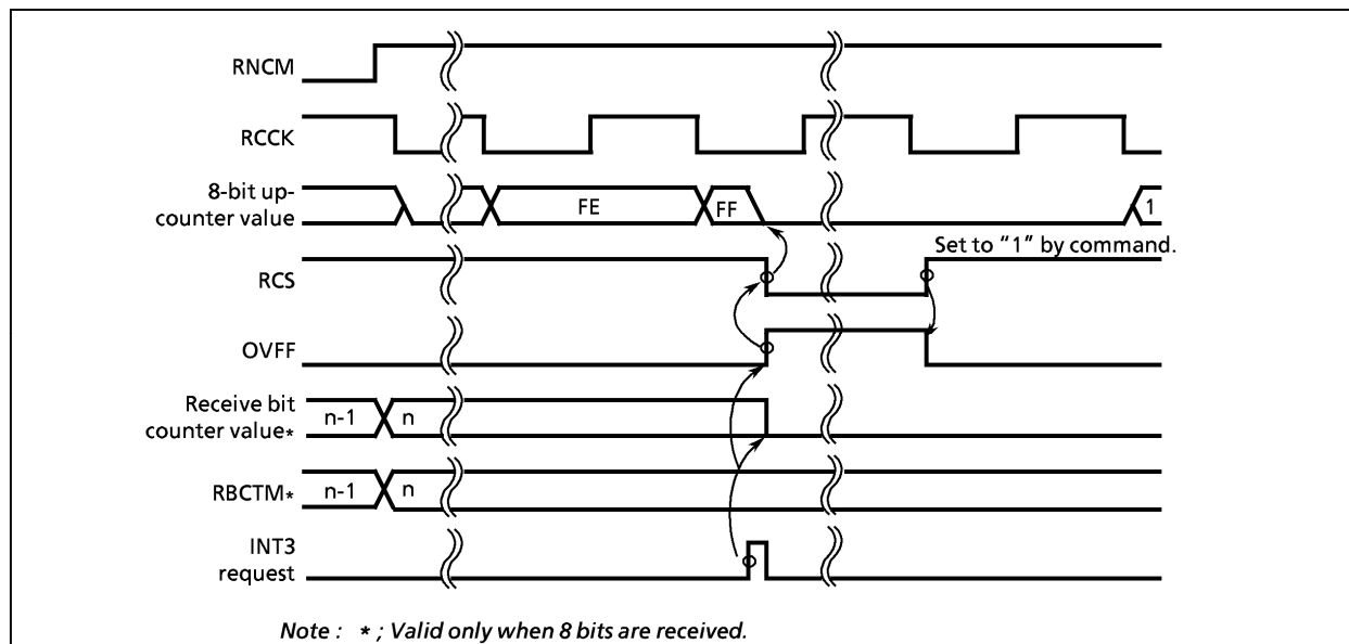
Figure 2-58. Overflow interrupt timing chart
