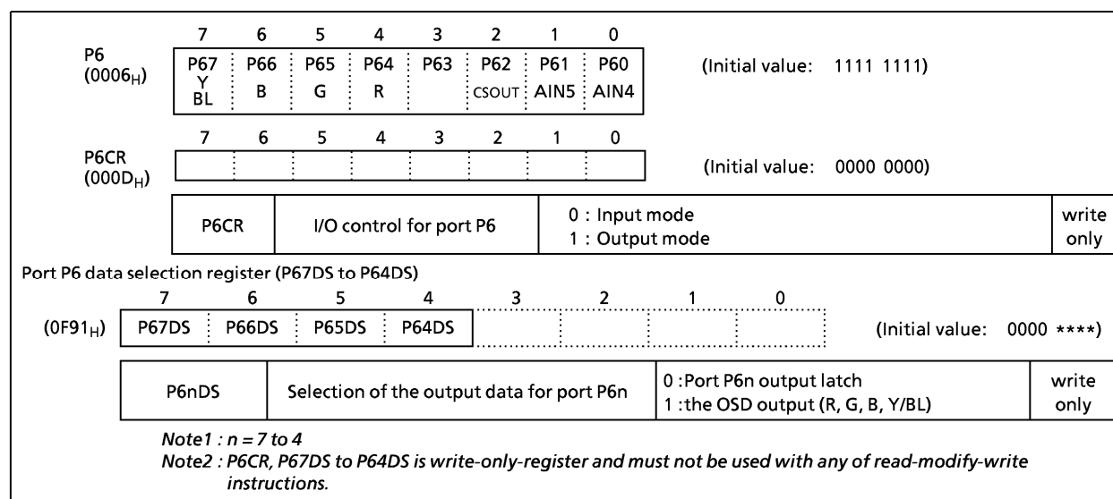
Figure 2-7-2. Ports P6, P6CR, and P67DS to P64DS
