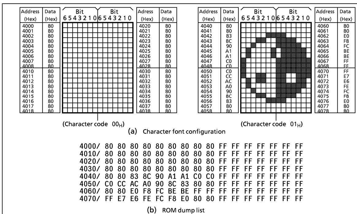
Figure 2-71. Character font configuration and ROM dump list
