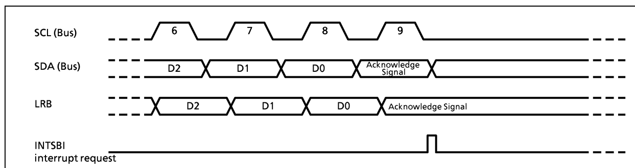
Figure 2-36. Last received bit monitor
