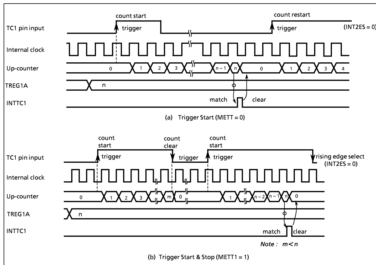
Figure 2-15. External trigger timer mode timing chart
