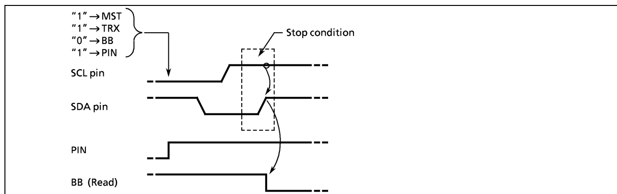
Figure 2-41. Stop condition generation
