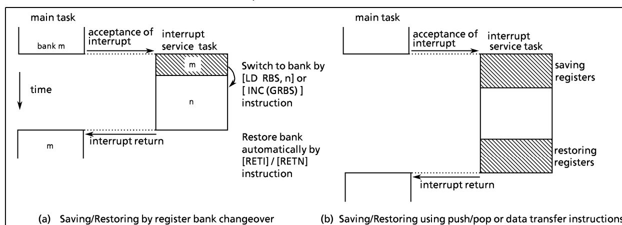
Figure 1-24. Saving/restoring general-purpose registers
