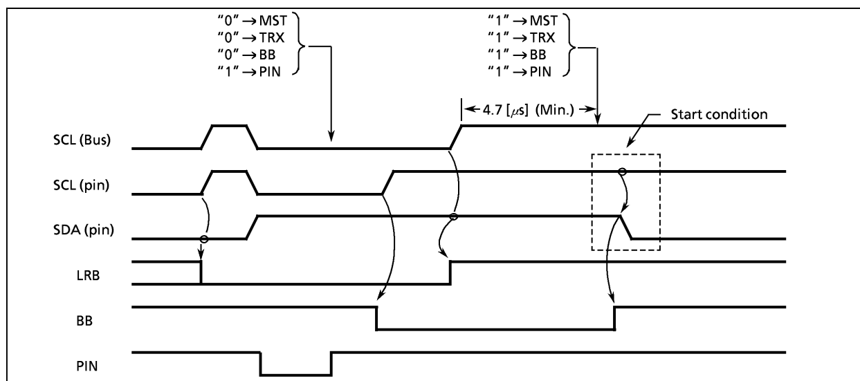
Figure 2-42. Timing diagram when restarting
