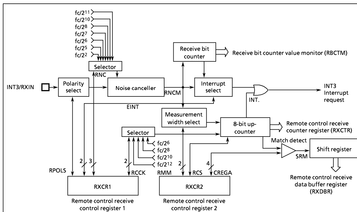
Figure 2-52. Remote control signal preprocessor
