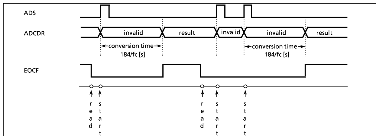
Figure 2-63. A/D conversion timing chart
