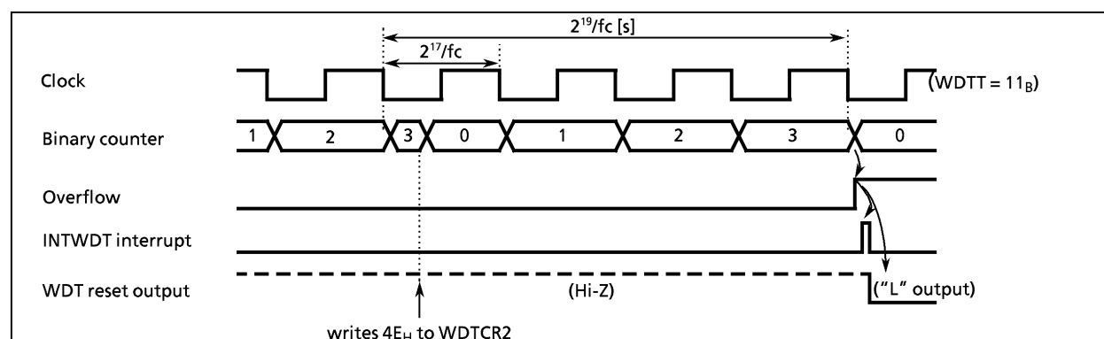
Figure 1-28. Watchdog timer interrupt / reset
