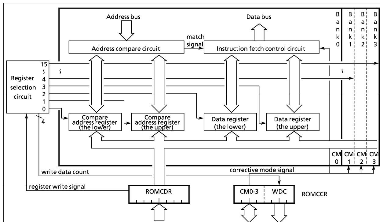
Figure 1-31. ROM correction circuit
