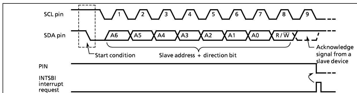
Figure 2-37. Start condition generation and slave address transfer
