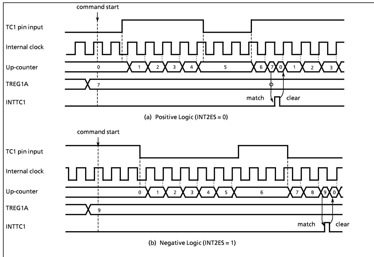
Figure 2-17. Window mode timing chart
