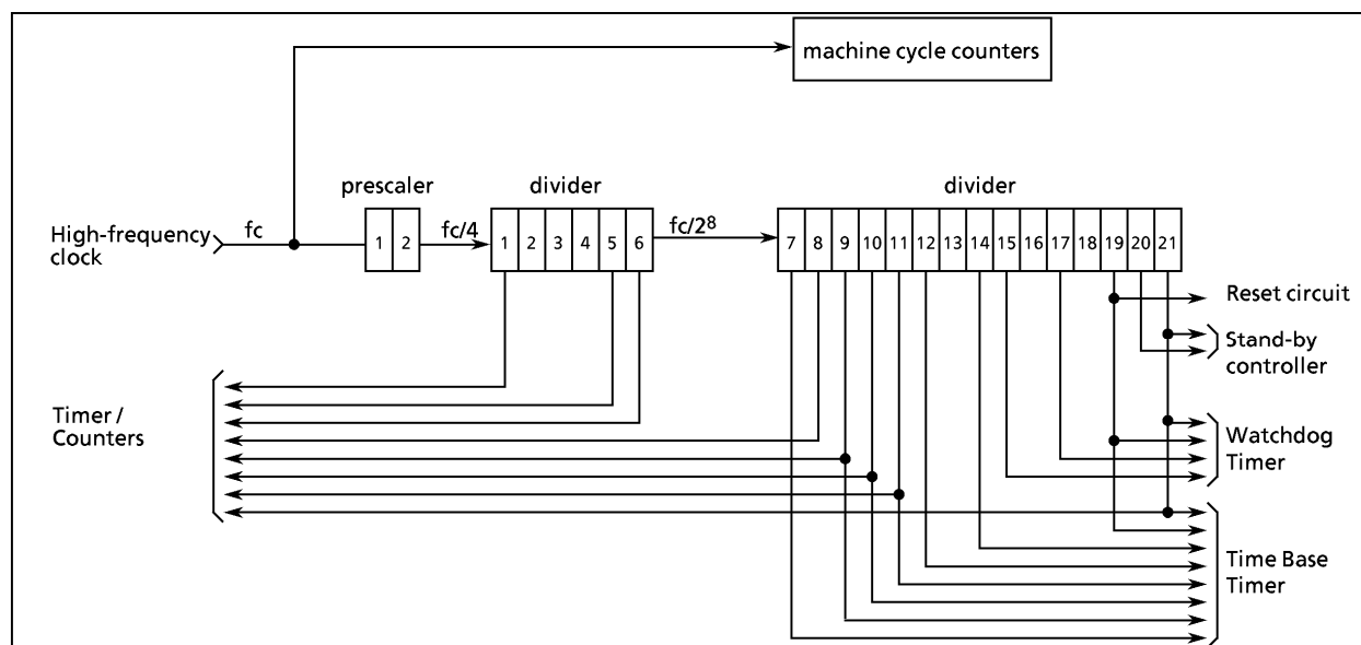
Figure 1-12. Configuration of timing generator
