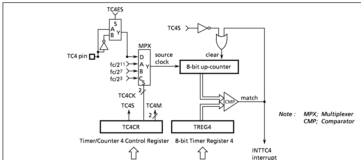
Figure 2-25. Timer / counter 4
