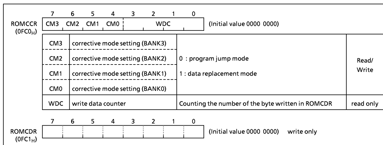
Figure 1-32. ROM corrective control register and ROM corrective data register
