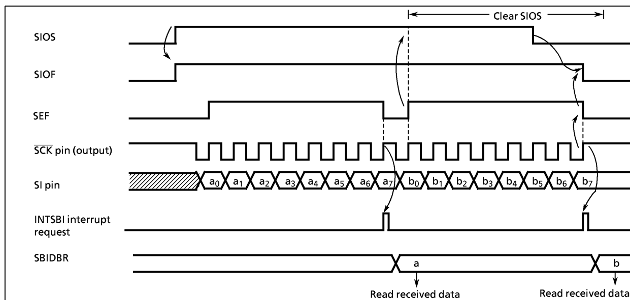
Figure 2-49. Receive mode (Example : Internal clock)
