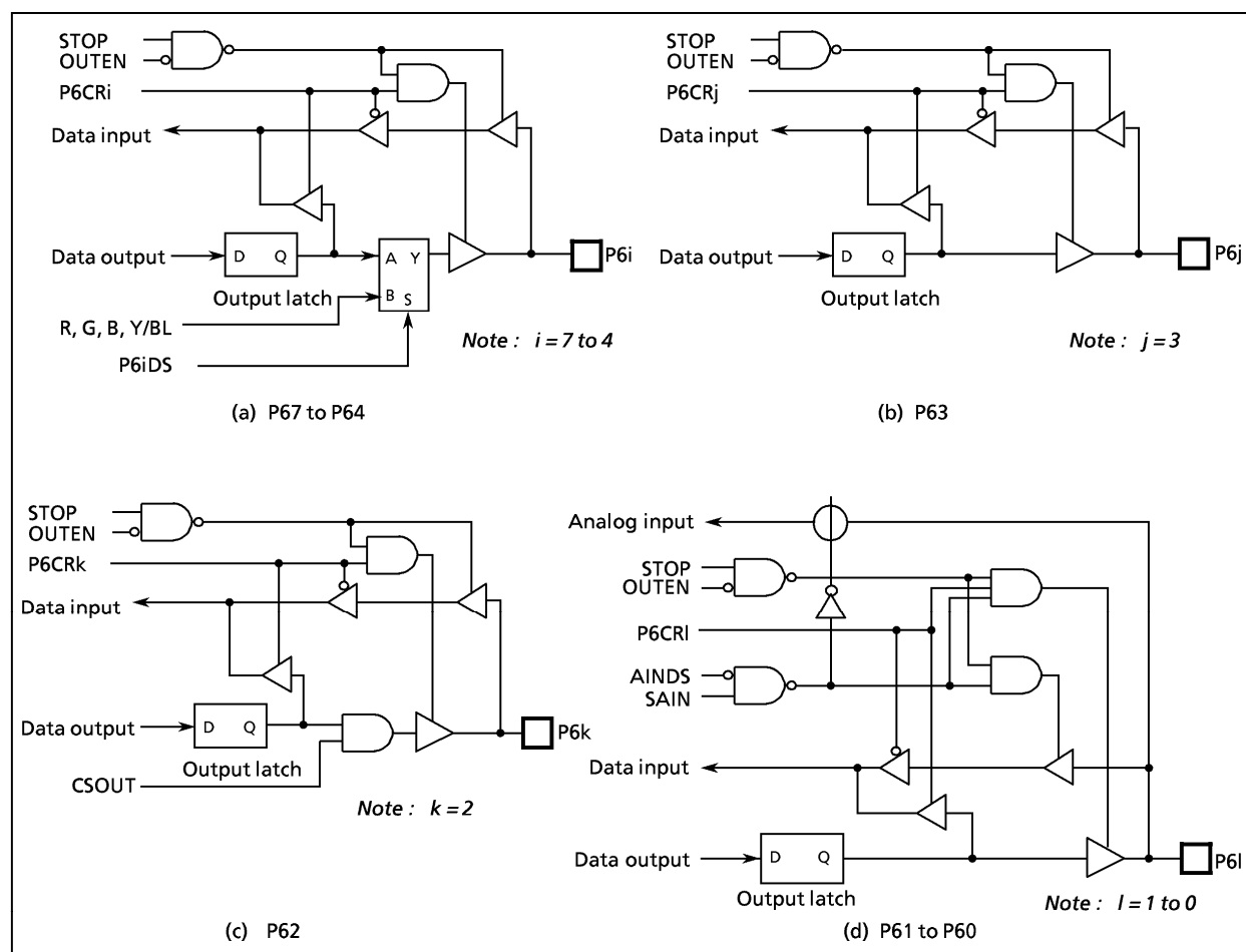
Figure 2-7-1. Ports P6, P6CR, and P67DS to P64DS
