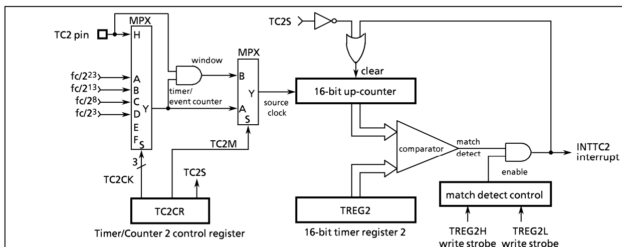
Figure 2-19. Timer/counter 2 (TC2)
