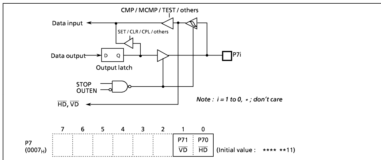
Figure 2-8. Ports P7
