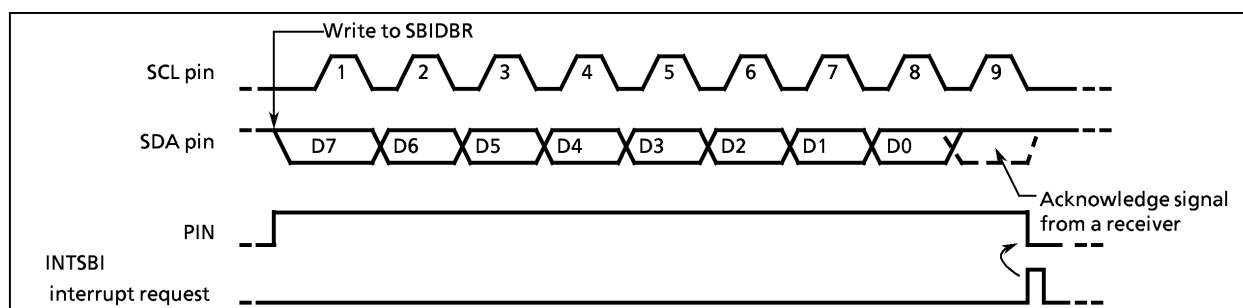
Figure 2-38. Example when BC = "000", ACK = "1" in transmitter mode
