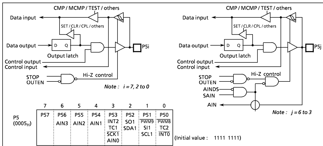
Figure 2-6. Ports P5
