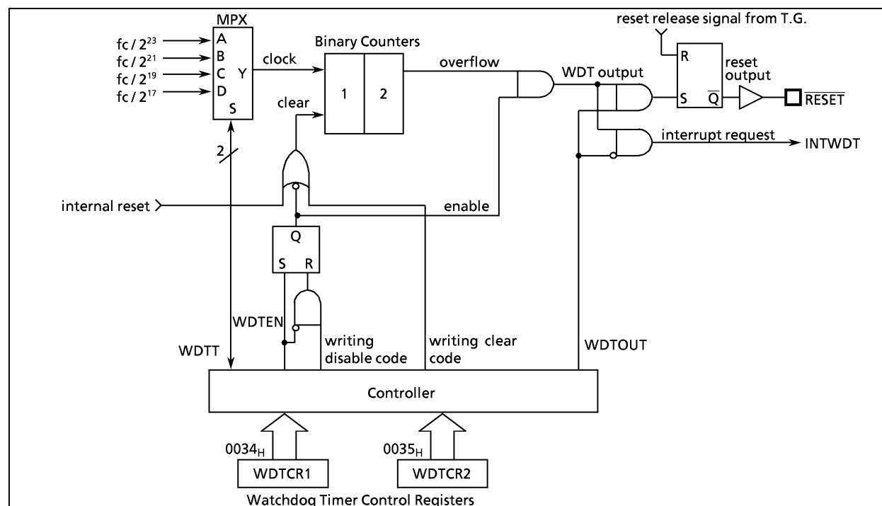
Figure 1-26. Watchdog timer configuration
