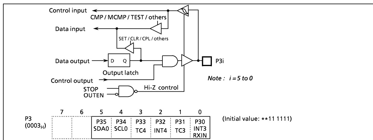
Figure 2-4. Port P3
