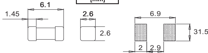
Dimensions [mm]
