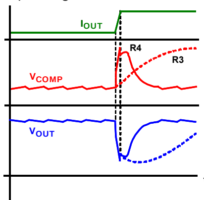
FIGURE 16. R^3 vs R^4 IDEALIZED TRANSIENT RESPONSE
