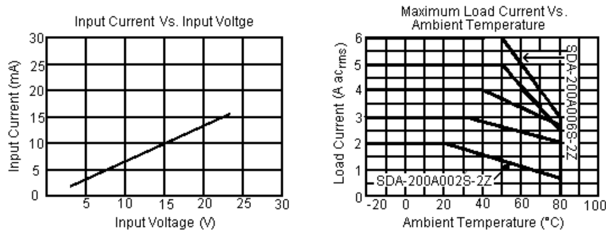
Characteristic Curves
