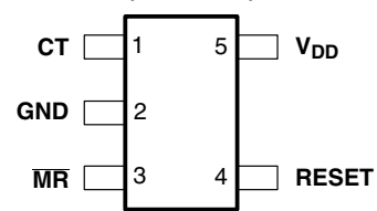
TPS3837 DBV PACKAGE (TOP VIEW)
