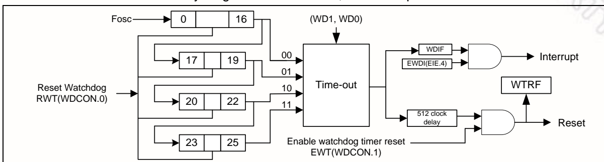
Figure 12-1 Watchdog Timer
