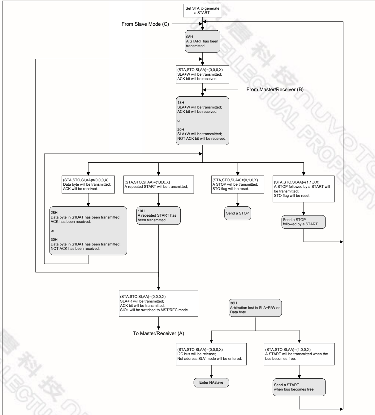
Figure 15-5 Master Transmitter Mode
