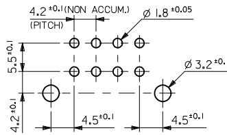
RECOMMENDED PCB HOLE LAYOUT VIEWED FROM COMPONENT SIDE 1.78 MAX. THICK P.C. BOARD
