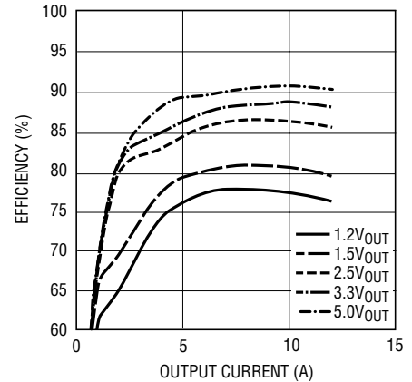
Efficiency vs Load Current with 20V IN
