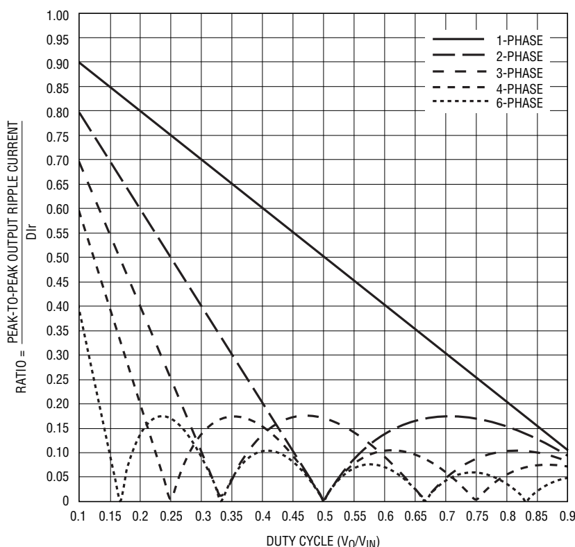
Figure 4. Normalized Output Ripple Current vs Duty Cycle, DIL = V_O T / L_I , DIL = Each Phase's Inductor Current
