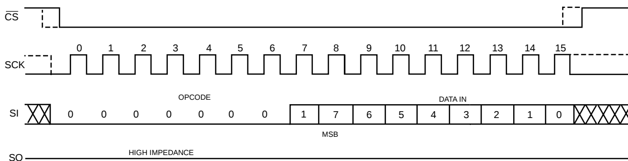
Figure 8. WRSR Timing
