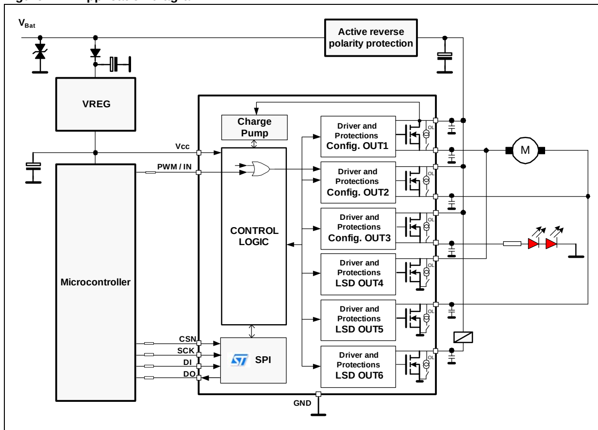
Figure 1. Application diagram
