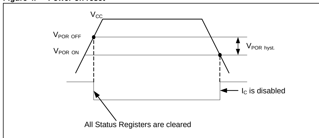
Figure 4. Power-on reset
