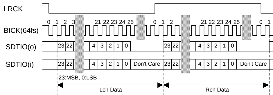
Figure 8. Mode 2 Timing
