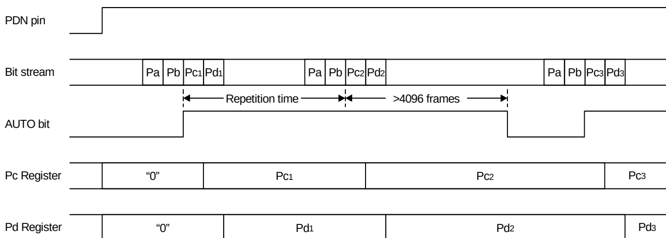
Figure 27. Timing example 1
