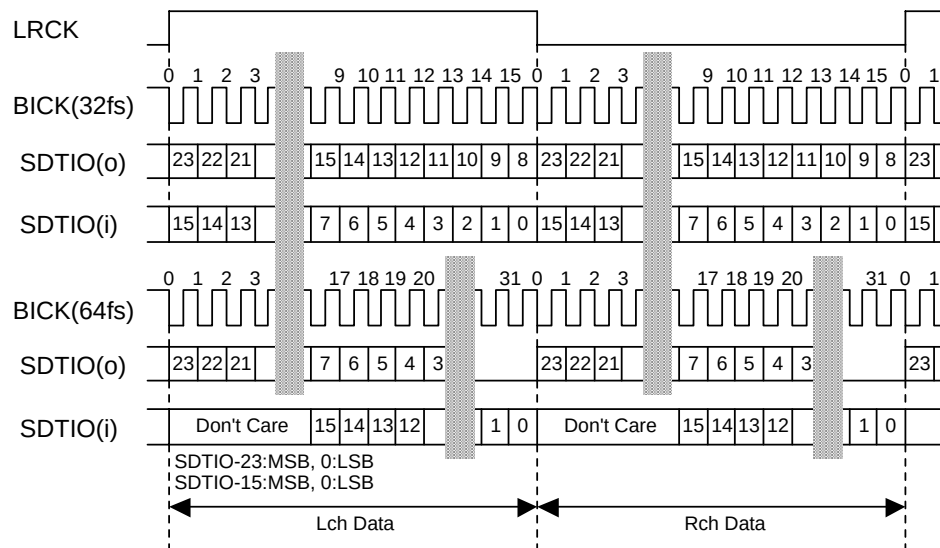
Figure 6. Mode 0 Timing
