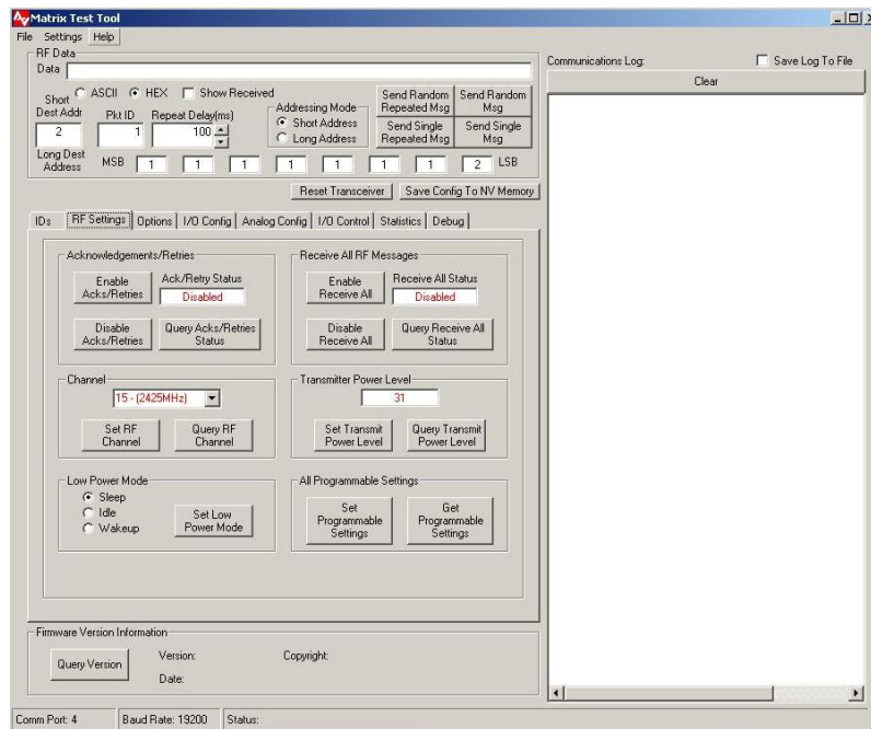
Figure 4-3. RF Settings
