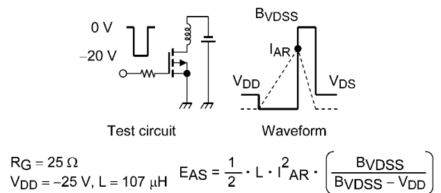
Fig. 8.15 Test Circuit/Waveform
