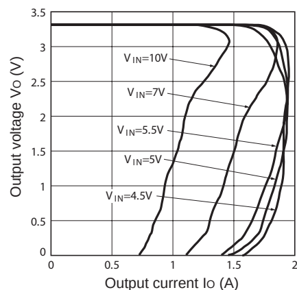
Fig.13 Overcurrent Protection Characteristics (PQ033EZ01ZxH)
