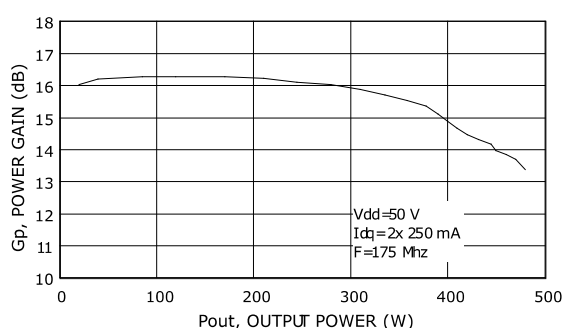
Figure 12: Power gain vs. output power
