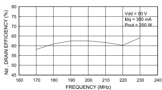
Figure 21: Efficiency vs. frequency
