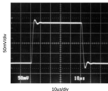
SMALL-SIGNAL STEP RESPONSE C_L = 1000\text{pF}
