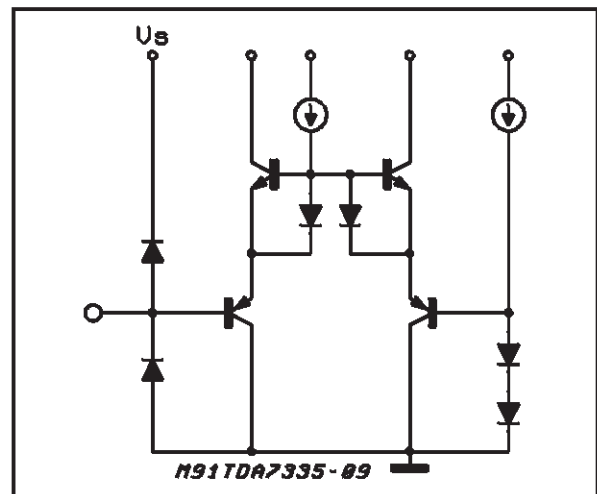
Figure 10: PINS: 5 - 26
