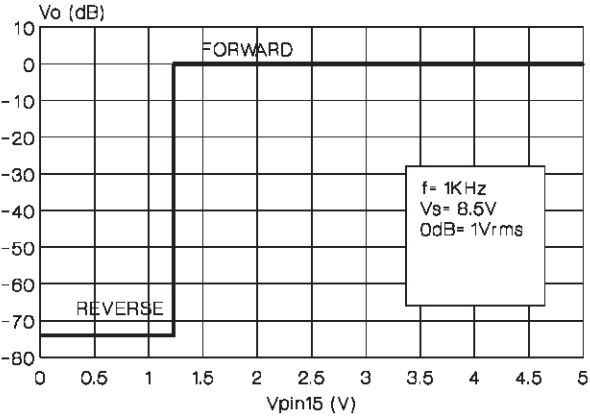
Figure 40: Load Characteristics
