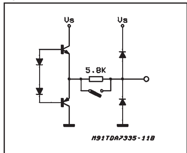
Figure 10: PINS: 5 - 26
