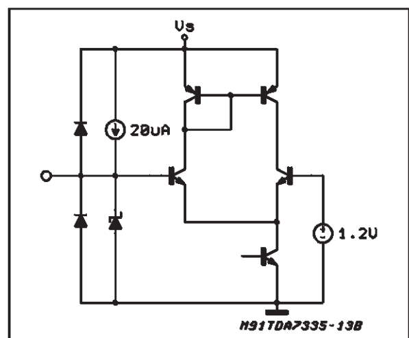
Figure 12: PINS: 8 - 15
