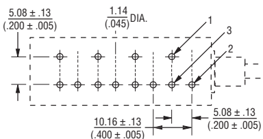
Model 81 Suggested PC Board Layout - PC Pins (Single-Shaft Style Bottom View)
