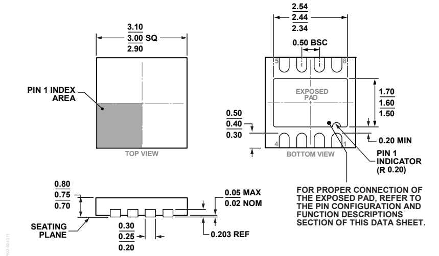
Figure 43. 8-Lead Lead Frame Chip Scale Package [LFCSP] 3 mm × 3 mm Body and 0.75 mm Package Height (CP-8-21) Dimensions shown in millimeters
