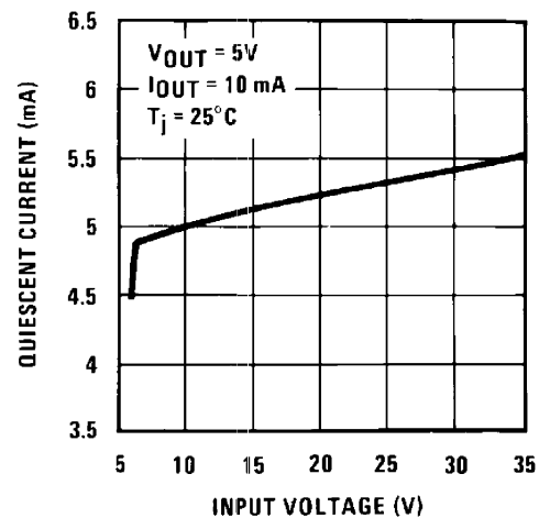
Figure 12. Quiescent Current
