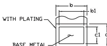
LEAD TIP DETAIL
