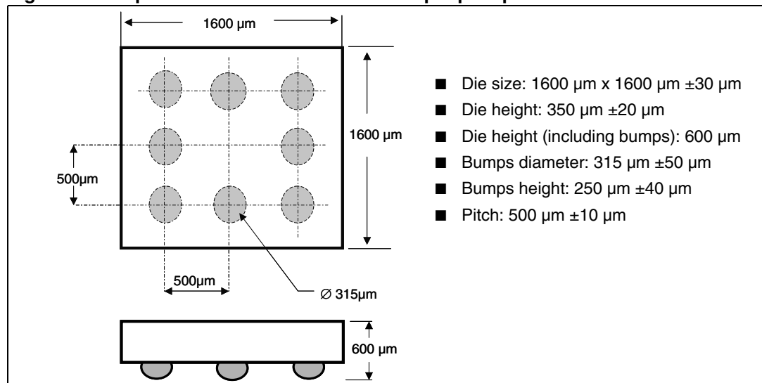
Figure 14. Top view and dimensions of 8-bump flip-chip
