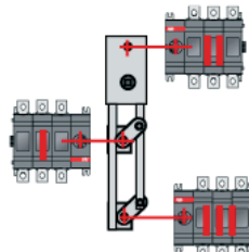
By-pass switches
