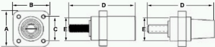
Panel Mount Receptacle; 1/2"-13 UNC Thread Stud
