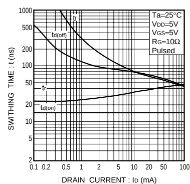
Fig.20 Switching characteristics
