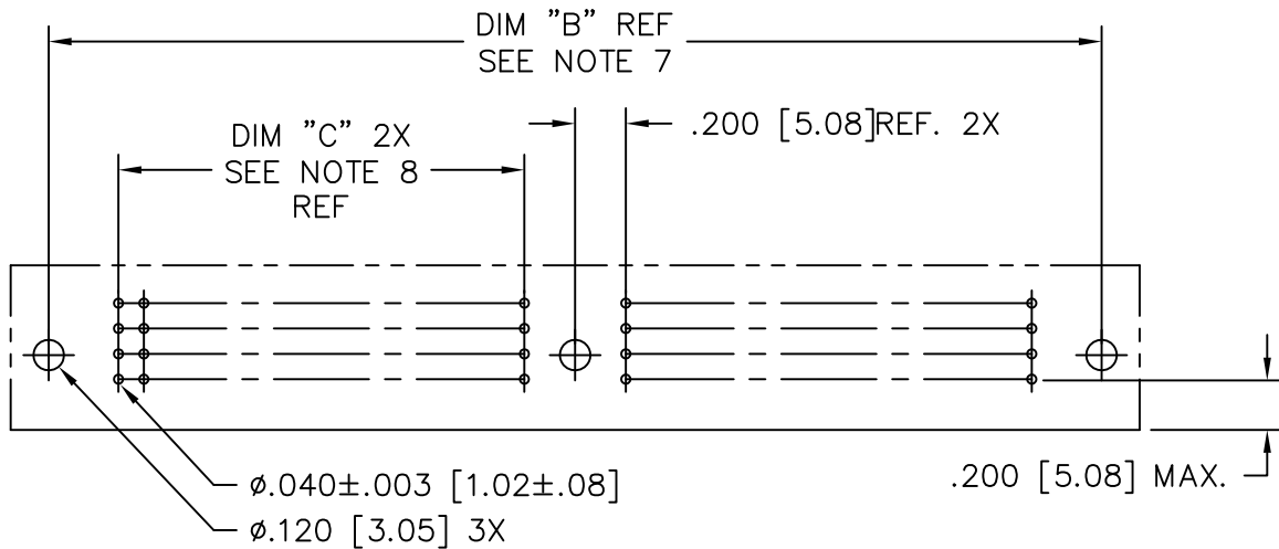
SECTION U-U
