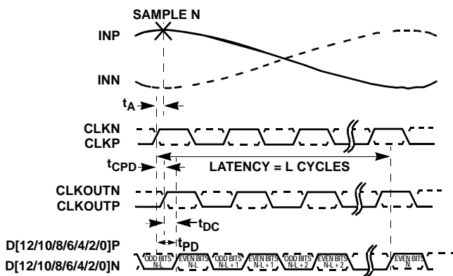
FIGURE 1A. DDR
