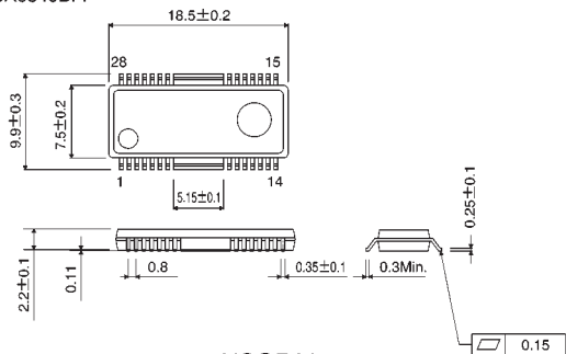
HSOP28
