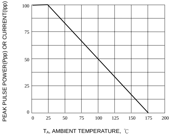
Fig. 2-PULSE DERATING CURVE
