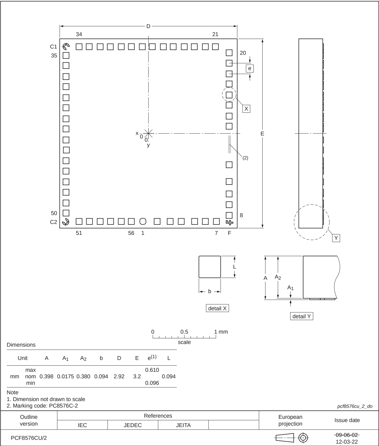
Fig 36. Bare die outline of PCF8576CU/2/F2
