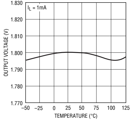
Output Voltage
