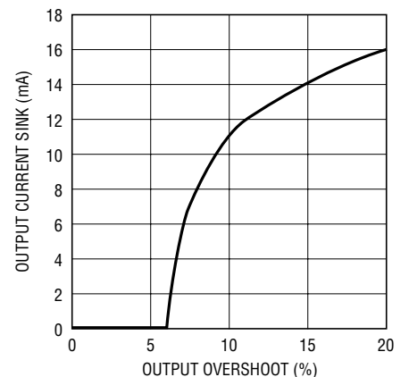
No-Load Recovery Threshold
