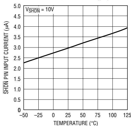
SHDN Pin Input Current ( \mu\text{A} )
