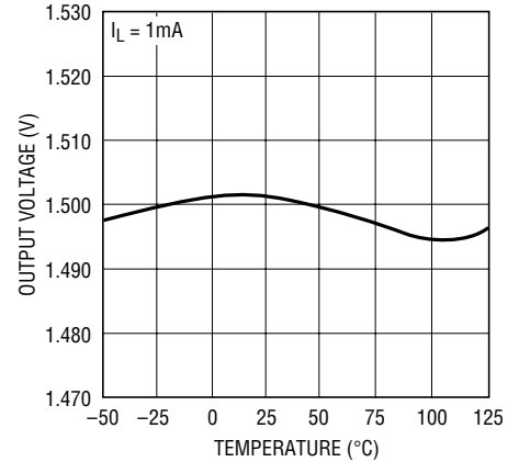
Output Voltage
