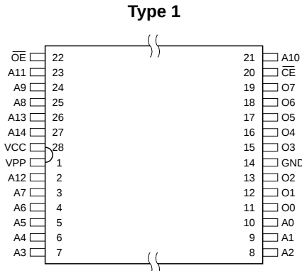
TSOP Type 1
