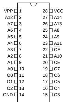
TSOP Type 1
