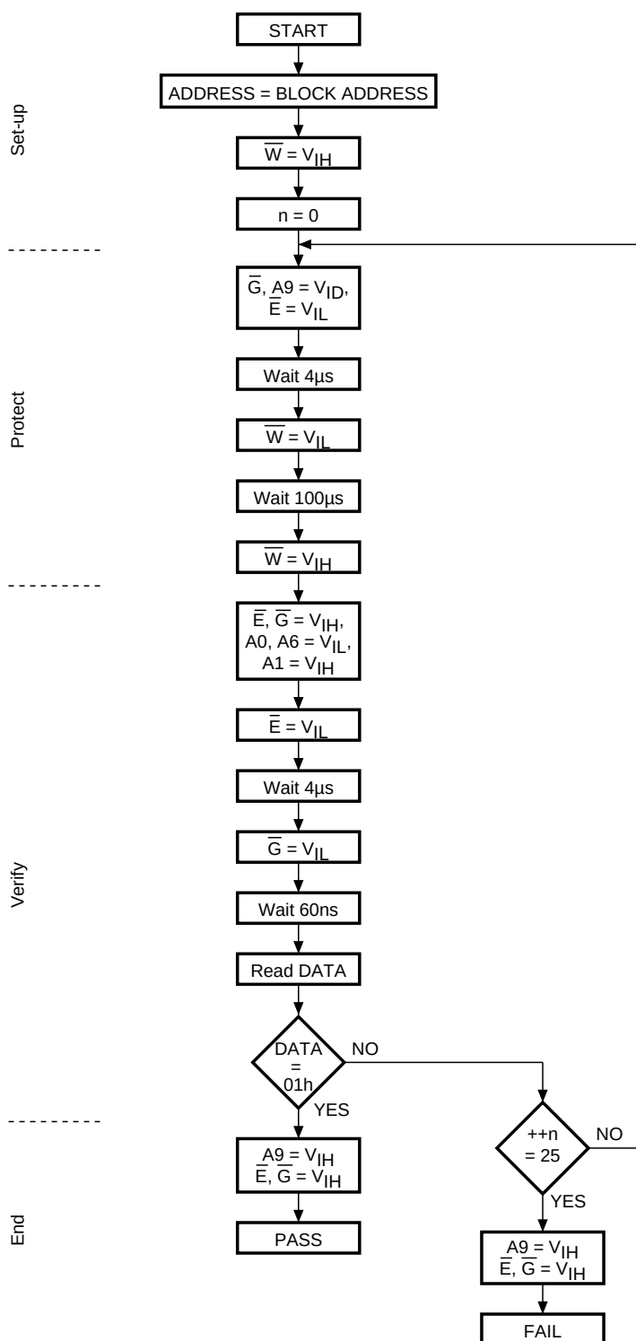
Figure 19. Programmer Equipment Block Protect Flowchart
