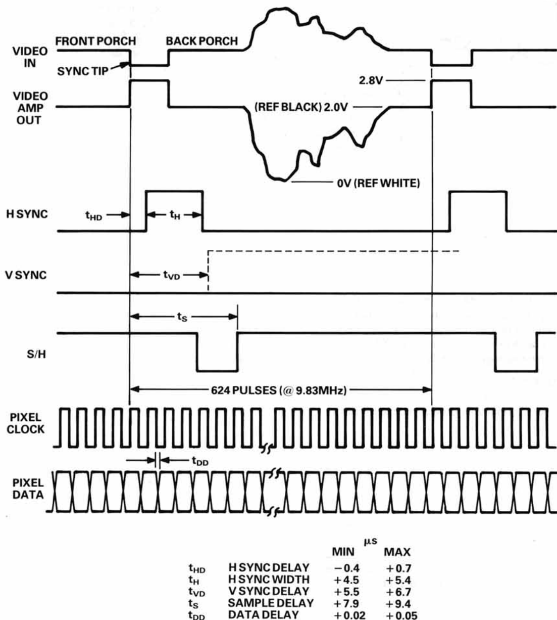
Figure 1. AD9502 Timing Diagram
