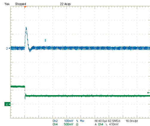
Step Load Transient Response (Vin=5V, Vout=1.8V, Load=0, Iout=3A to 1.5A) Trace 2=Vout, 100 mV/div. Trace 4=Iout, 2.5A/div.
