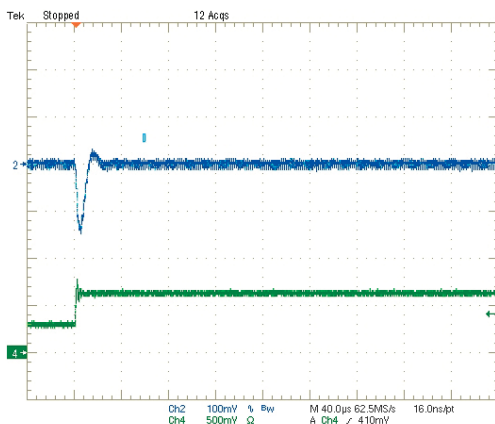
Step Load Transient Response (Vin=5V, Vout=1.2V, Load=0, Iout=1.5A to 3A) Trace 2=Vout, 100 mV/div. Trace 4=Iout, 2.5A/div.
