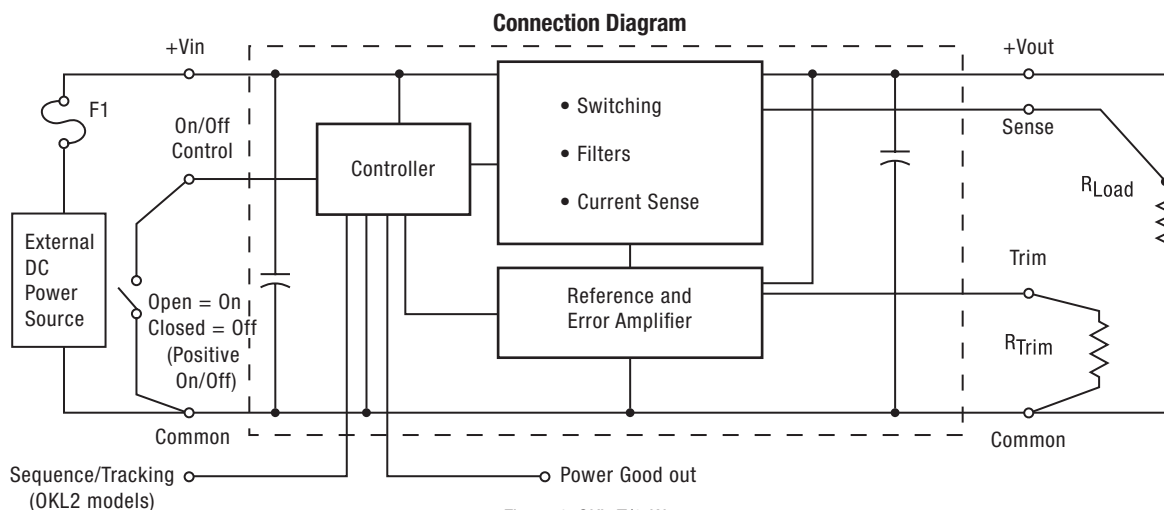
Figure 1. OKL-T/3-W5
