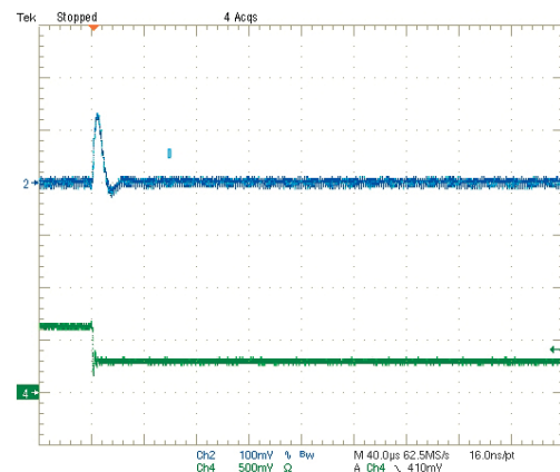
Step Load Transient Response (Vin=5V, Vout=1.2V, Load=0, Iout=3A to 1.5A) Trace 2=Vout, 100 mV/div. Trace 4=Iout, 2.5A/div.
