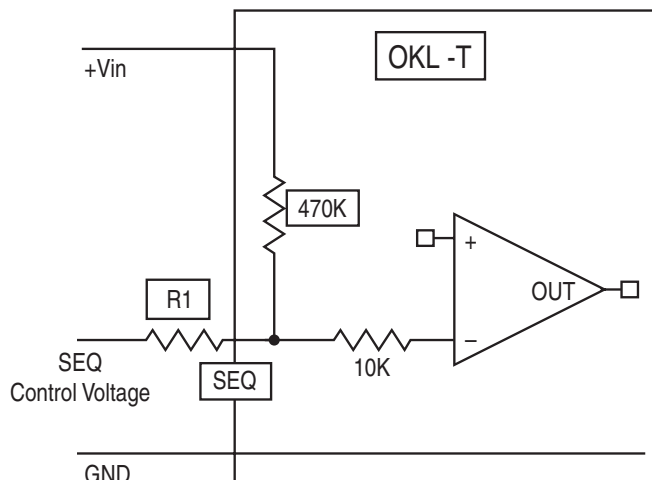
Figure 6. Sequencing Signal Interface of Module
